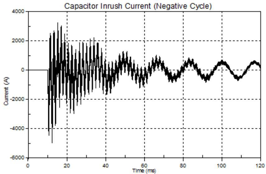
Figure 6.14. Capacitor Inrush Current (Negative Cycle)
