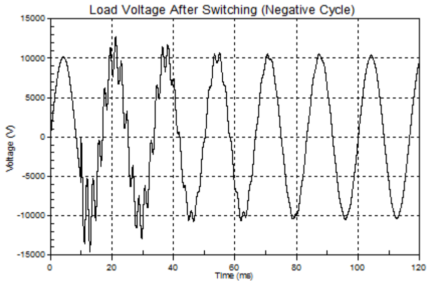
Figure 6.15. Load Voltage after Switching (Negative Cycle)
