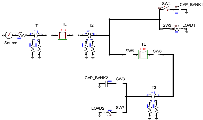
Figure 2.3. One-line Diagram for 3 \Phi Capacitor Switching Analysis
