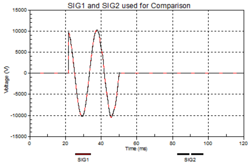
Figure 5.6. SIG_1 and SIG_2 used to find Zero Crossing
