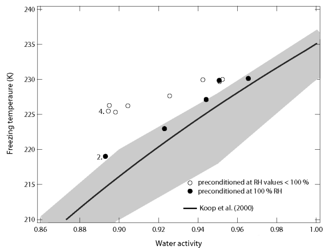
Fig. 5. Freezing temperature versus water activity for ammonium sulfate particles preconditioned at RH values < 100% (open circles) and preconditioned at 100% RH (filled circles). For comparison, freezing temperatures predicted using the water activity based nucleation theory developed by Koop et al. (2000) are shown as a solid line. The spread in the data points used to construct the solid line is represented by the shaded area. The IR spectra shown in Fig. 2 were used to produce the point highlighted with the “2” and the IR spectra shown in Fig. 4 were used to produce the point highlighted with the “4”.
