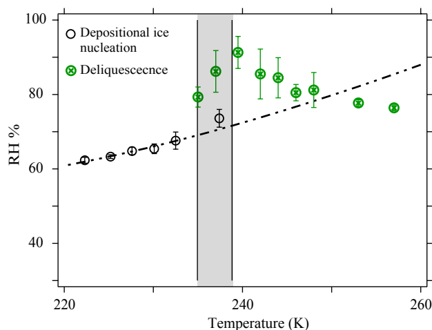
Fig. 9. Relative humidity versus temperature for depositional ice nucleation on hydrated NaCl (s) (open circles) and deliquescence of hydrated NaCl (s) (crossed green circles). The grey shading denotes the temperatures at which both depositional ice nucleation and deliquescence occur. The dashed-dotted line represents RH at an S_{ice} = 1 .
