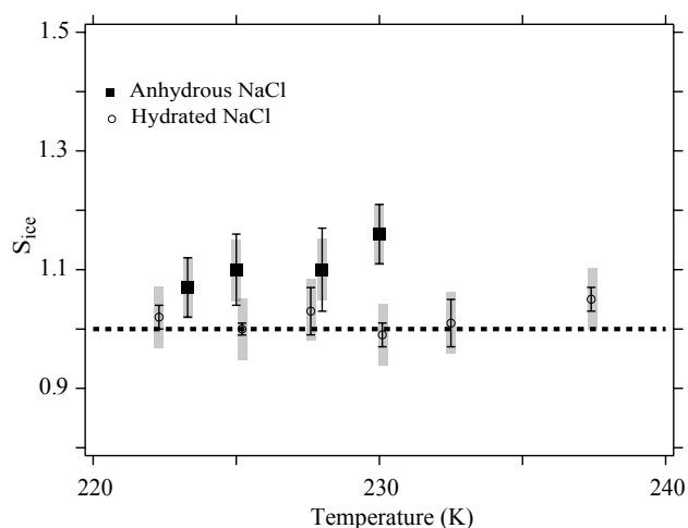
Fig. 8. S_{ice} versus temperature for the onset of depositional ice nucleation on NaCl (solid squares) and hydrated NaCl particles (open circles). An S_{ice} of 1 is denoted with the dotted line. Here, depositional ice nucleation is defined as the onset of ice nucleation and represents the conditions at which the first particle on the substrate nucleated ice. The error range (represented by the lines) is the high and low value for each bin. Additionally, the grey error bars represent experimental error.
