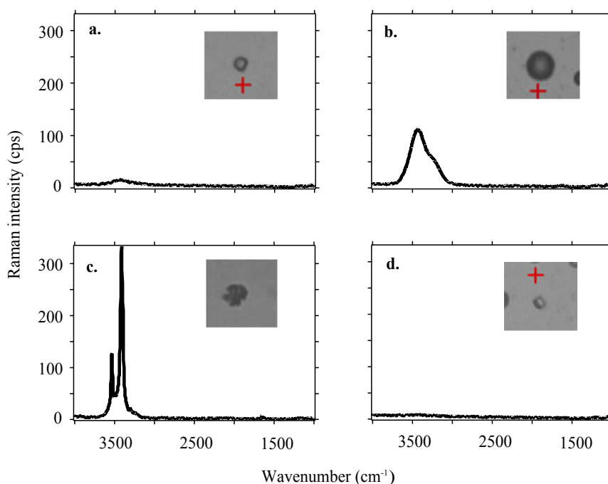
Fig. 2. Raman spectra of the particles highlighted in Fig. 1.
