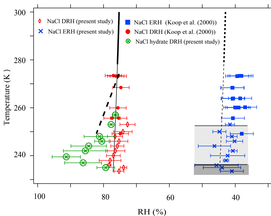
Fig. 5. NaCl phase diagram adapted from Koop et al. (2000): NaCl ERH (solid blue squares), NaCl DRH (solid red circles), high temperature NaCl DRH (solid black vertical line), high temperature NaCl ERH (dotted black vertical line), theoretical NaCl hydrate DRH (thick black dashed line). Data collected from the present study: NaCl hydrate DRH (crossed green circles), NaCl DRH (open red diamonds), NaCl ERH (blue crosses), region where mixed particles effloresce (light gray shade), region where hydrated particles effloresce (dark gray shade).
