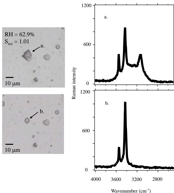
Fig. 7. Depositional ice nucleation experiment performed at 224 K on a mixed hydrated/anhydrous \text{NaCl}_{(s)} sample. Particle (a) in the top left image is an ice particle which nucleated on a hydrated \text{NaCl}_{(s)} particle at an S_{\text{ice}} value of 1.01. Particle (b) in the lower left image is the ice nucleus after the ice was sublimed. Raman spectra of both particles were taken to confirm the presence of ice and the hydrated \text{NaCl}_{(s)} particle.
