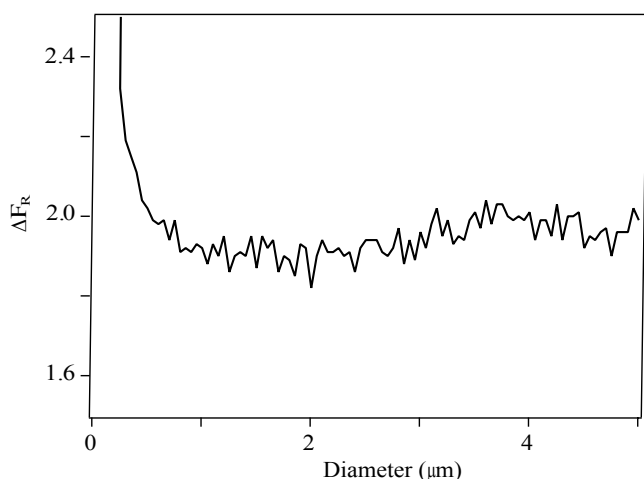
Fig. 11. Ratio of the radiative forcing of hydrated NaCl particles with respect to dry particles ( \Delta F_R ) as a function of particle diameter.
