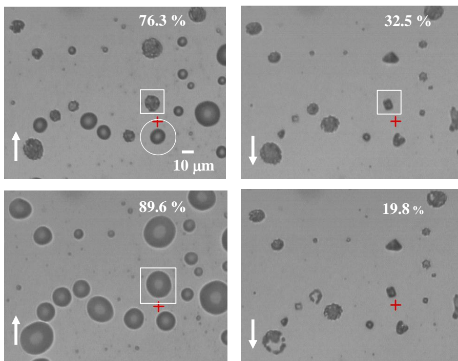
Fig. 4. NaCl particles (at 50X magnification) at 244 K as RH is cycled a second time. The up arrows indicate that water is being added to the environmental cell and the down arrows indicate that water is being removed from the environmental cell.
