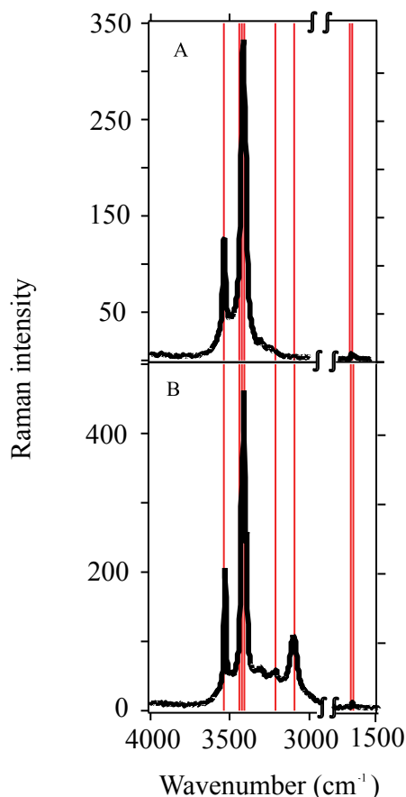
Fig. 3. (A) Raman spectrum of the non-cubic form of solid NaCl collected at 244 K. (B) Raman spectrum of the non-cubic form of solid NaCl collected at 163 K. The solid vertical lines highlight the peaks in the Raman spectrum collected by Dubessy et al. (1982) supposedly for solid sodium chloride dihydrate. The middle portion of the Raman spectrum has been removed because no peaks are present.
