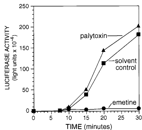
FIG. 2. Effect of palytoxin on the translation of luciferase mRNA in a rabbit reticulocyte lysate assay. The mRNA for luciferase (0.5 \mu g), palytoxin (30 nM), or solvent ( \text{H}_3\text{C}_2\text{SO} ) was added at t = 0 min. Emetine (10 \mu g/ml) was added at t = 8 min. At designated times, aliquots of the lysate were withdrawn and analyzed for luciferase activity. The assay was performed with a reticulocyte lysate kit, supplemented with amino acids, as described by the manufacturer (Promega).
