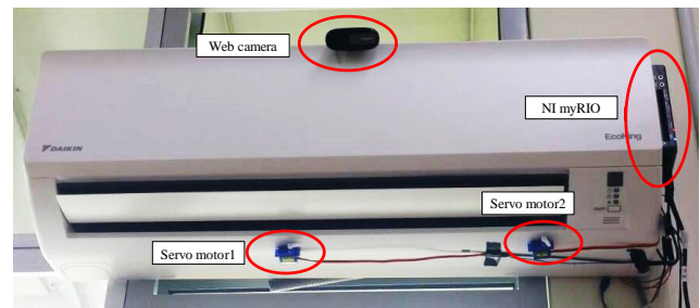
Figure 7: Real implementation of the dynamic tracking mechanism
