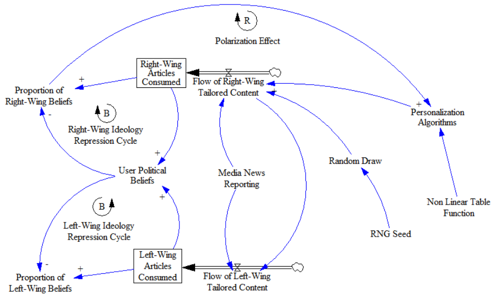
Figure 2. Stock and Flow Diagram
