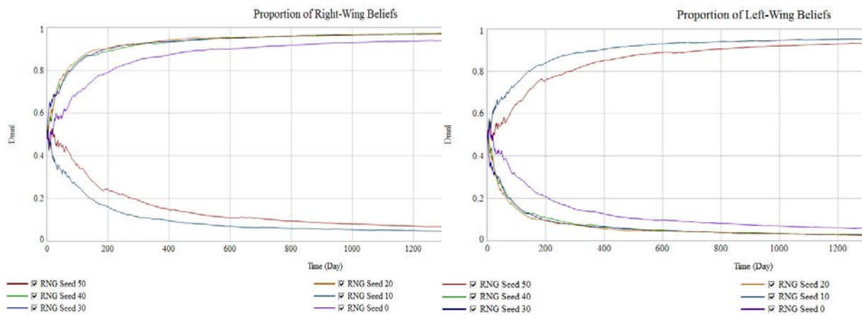
Figure 7. Proportion of Left-Wing Beliefs and Proportion of Right-Wing Belief RNG Seed Sensitivity
