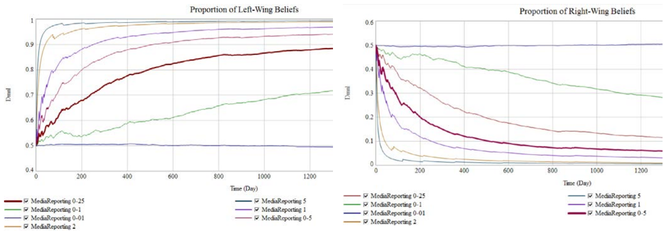
Figure 9. Proportion of Left-Wing Beliefs and Right-Wing Beliefs Media News Reporting Sensitivity
