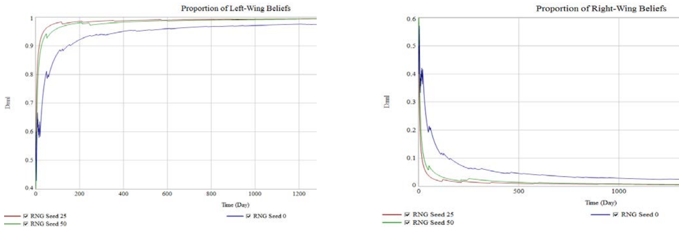
Figure 3. Effects of RNG Seed Extreme Conditions Testing on Proportion of Left and Right-Wing Beliefs
