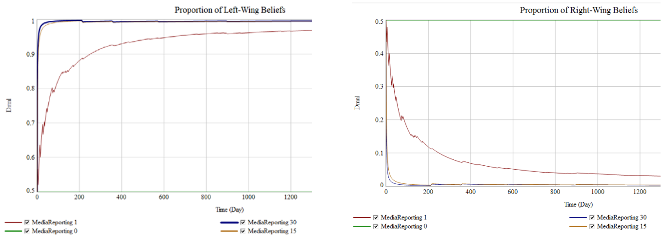
Figure 5. Effects of Media News Reporting Extreme Conditions Testing on the Proportion of Left-Wing Beliefs and the Proportion of Right-Wing Beliefs
