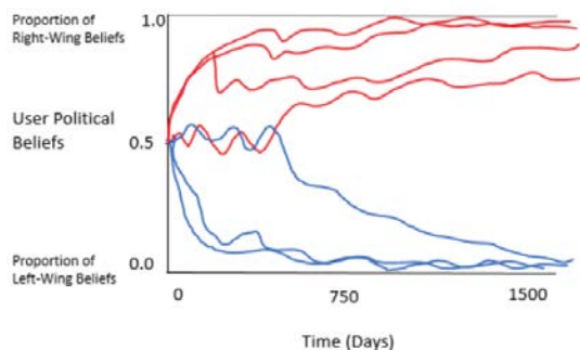
Figure 1. Reference Mode of Proportion of Right-Wing Beliefs
