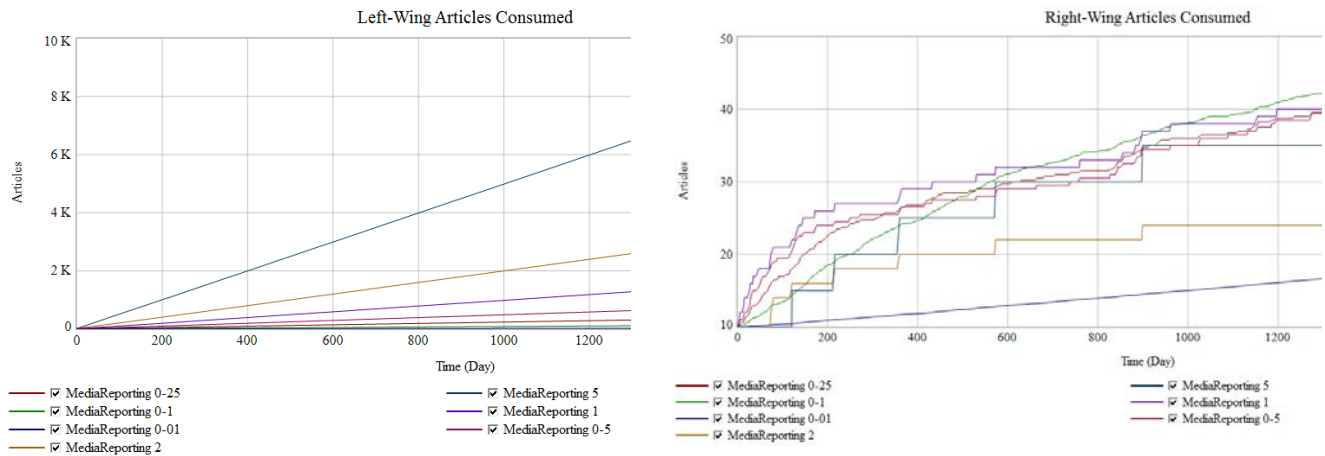
Figure 10. Left-Wing Articles Consumed and Right-Wing Articles Consumed Media News Reporting Sensitivity
