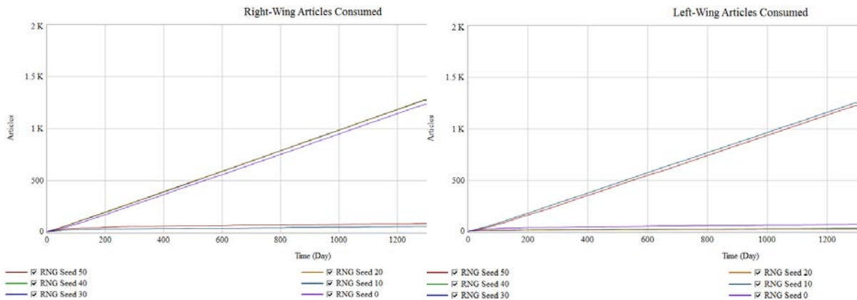
Figure 8. Right-Wing Articles Consumed RNG Seed Sensitivity
