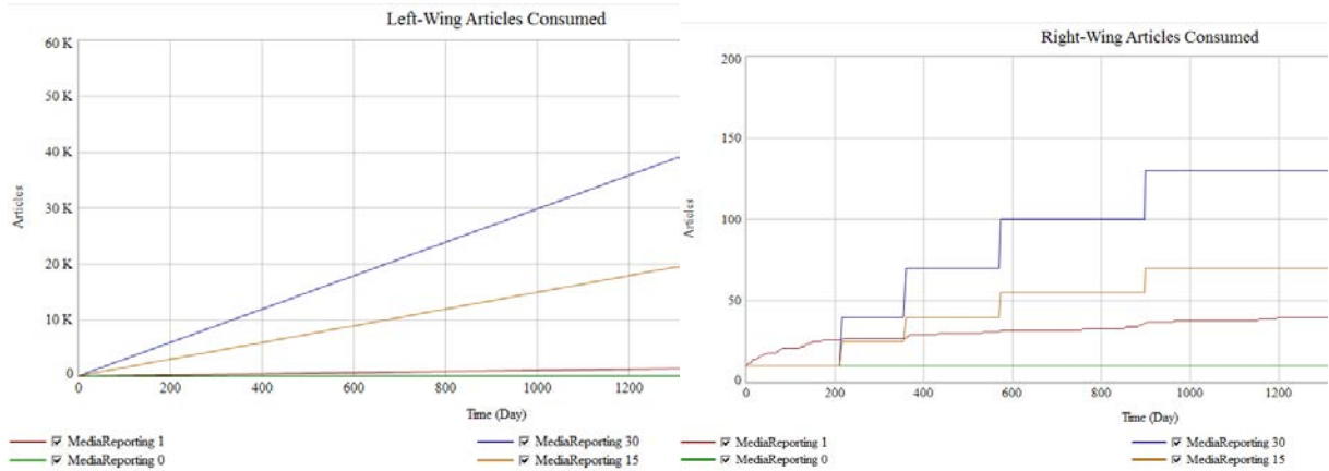
Figure 6. Effects of Media News Reporting Extreme Conditions Testing on Right-Wing Articles Consumed
