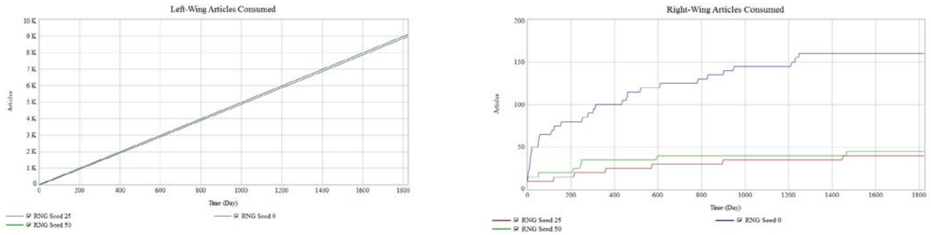
Figure 4. Effects of RNG Seed Extreme Conditions Testing on Left-Wing and Right-Wing Articles Consumed
