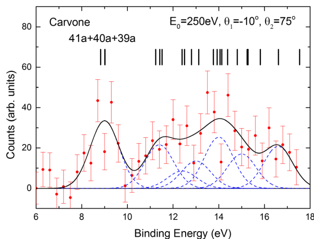
FIG. 2. The measured (e,2e) binding energy spectrum for R -carvone. This was obtained at an incident electron energy of E_0 = 250 eV by scanning over a range of detection energies for a fast electron scattered through an angle of -10^\circ . Here, the slow ejected electron was detected with an energy of E_2 = 20 eV and at a scattering angle of 75^\circ . The positions of the OVGf ionization energies for the dominant equatorial (eq-1) conformer are also shown. Also shown are the spectral deconvolution for the resolved orbital features (dashed lines) and their sum (solid line). See text for further details.
