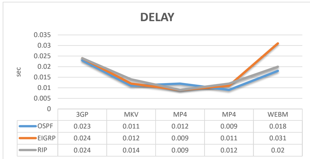
Gambar 3. Perbandingan Delay routing OSPF, EIGRP dan RIP
