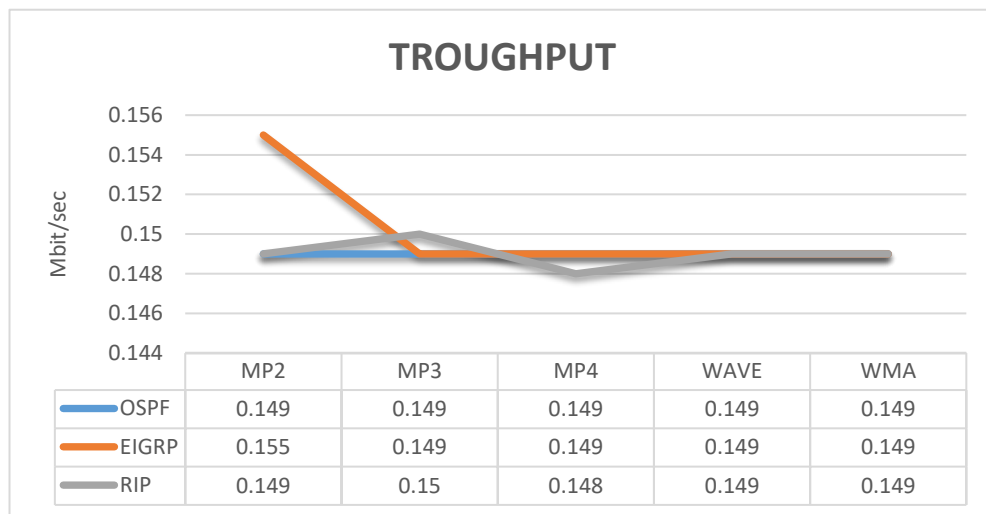
Gambar 5. Perbandingan Troughput Audio routing OSPF, EIGRP dan RIP
