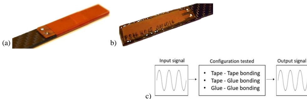
Figure 14: Bonding of rectangular piezo patch to the composite beam with special flash tape (a) and epoxy resin, as recommended by PI (b). Coupling effect study with different bonding configuration (c).
