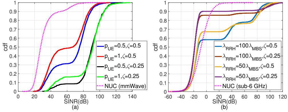
Fig. 6: Downlink SINR cdf comparison between user-centric S-cell and non user-centric PPP approaches in (a) single-tier and (b) multi-tier networks.
