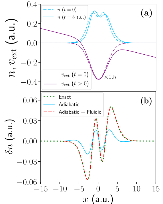
FIG. 1. System 1: Two interacting electrons in a Gaussian potential well, with a uniform electric field applied at t = 0 , driving the electrons to the right and inducing a current. (a) The ground-state external potential (dashed purple) and exact ground-state electron density (dashed blue), along with the perturbed external potential (solid purple) and exact time-dependent electron density at t = 8 a.u. (solid blue). (b) The change in the exact electron density [ \delta n(x, t) = n(x, t) - n(x, 0) ] at t = 8 a.u. (short-dashed green), along with that obtained when using the exact v_{\text{KS}}^{\text{A}} (solid blue), and when adding the exact v_{\text{KS}}^{\text{A}} with the fluidic approximation \Delta A_{\text{KS}} = -u (dashed red). The exact adiabatic potential is clearly inadequate, but its error is substantially reduced by the fluidic approximation.
