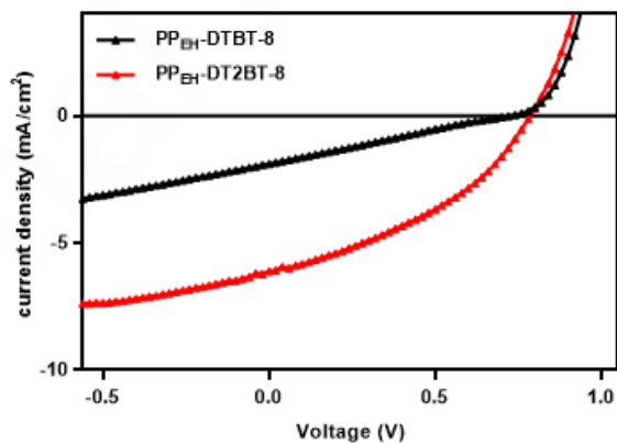
Figure 5: The J-V characteristic curves of PP_{EH-DTBT-8} and PP_{EH-DT2BT-8} .
