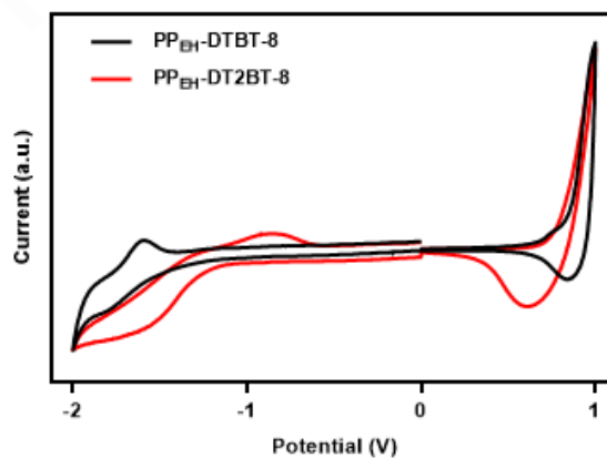
Figure 3. Cyclic voltammograms of thin films of PP EH -DTBT-8 and PP EH -DT2BT-8 on platinum disc electrodes (area 0.031 cm 2 ).
