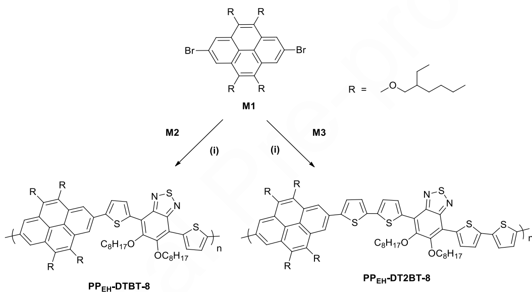
Scheme 2: Synthetic route and chemical structures of PEH-DTBT-8 and PEH-DT2BT-8 : (i) Pd(OAc) 2 , tri( o -tolyl)phosphine and toluene.
