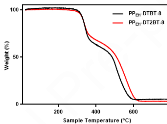
Figure 2: TGA curves of PP EH -DTBT-8 and PP EH -DT2BT-8.
