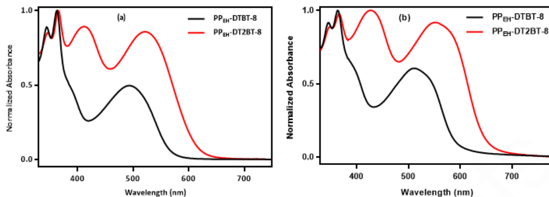
Figure 1. Normalised absorption spectra of PP EH -DTBT-8, PP EH -DT2BT-8, in: (a) chloroform solution; and (b) thin film.
