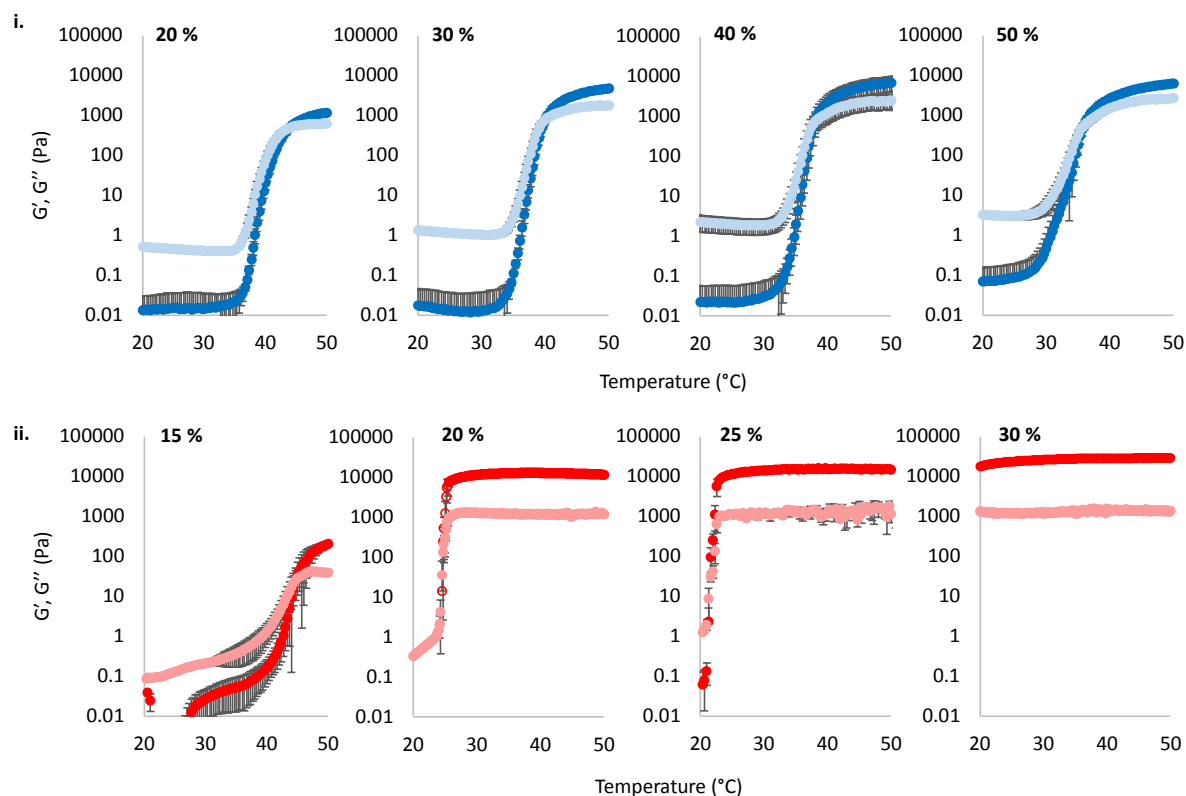
Figure 2. Temperature ramp rheograms of PNIPAM 98 -PEG 122 -PNIPAM 98 (i) and poloxamer 407 (ii) with variation of concentration (% w/v) at a fixed shear stress (1 Pa) and frequency (1 Hz). G' is presented as the dark colour, whilst the light colour corresponds to G'' . Data presented as mean \pm standard deviation, n = 3 .
