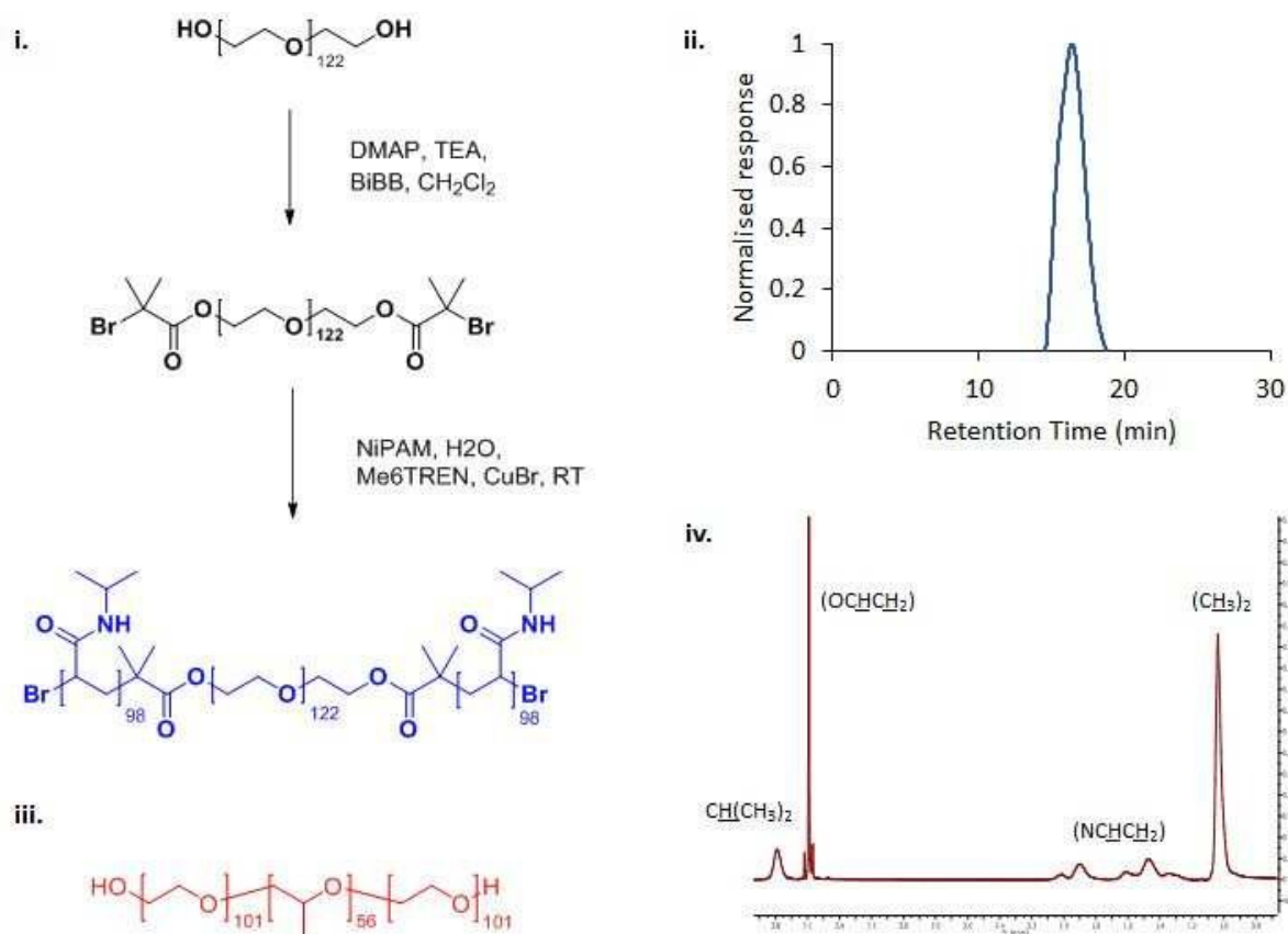
Figure 1. The synthetic route to PNIPAM 98 -PEG 122 -PNIPAM 98 (i) and chemical structure of poloxamer 407 (iii). PNIPAM 98 -PEG 122 -PNIPAM 98 was characterised by GPC (ii) and 1 H NMR (iv).
