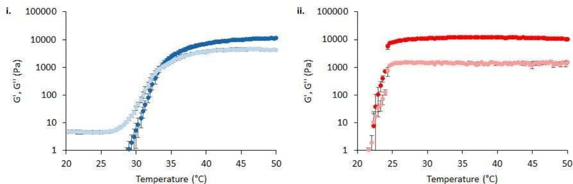
Figure 5. Temperature ramp rheograms of 50 % (w/v) PNIPAM 98 -PEG 122 -PNIPAM 98 (i) and 20 % (w/v) poloxamer 407 (ii) in VFS at a fixed shear stress (1 Pa) and frequency (1 Hz). G' and G'' are shown as dark and light markers, respectively. Data presented as mean \pm standard deviation, n = 3 .
