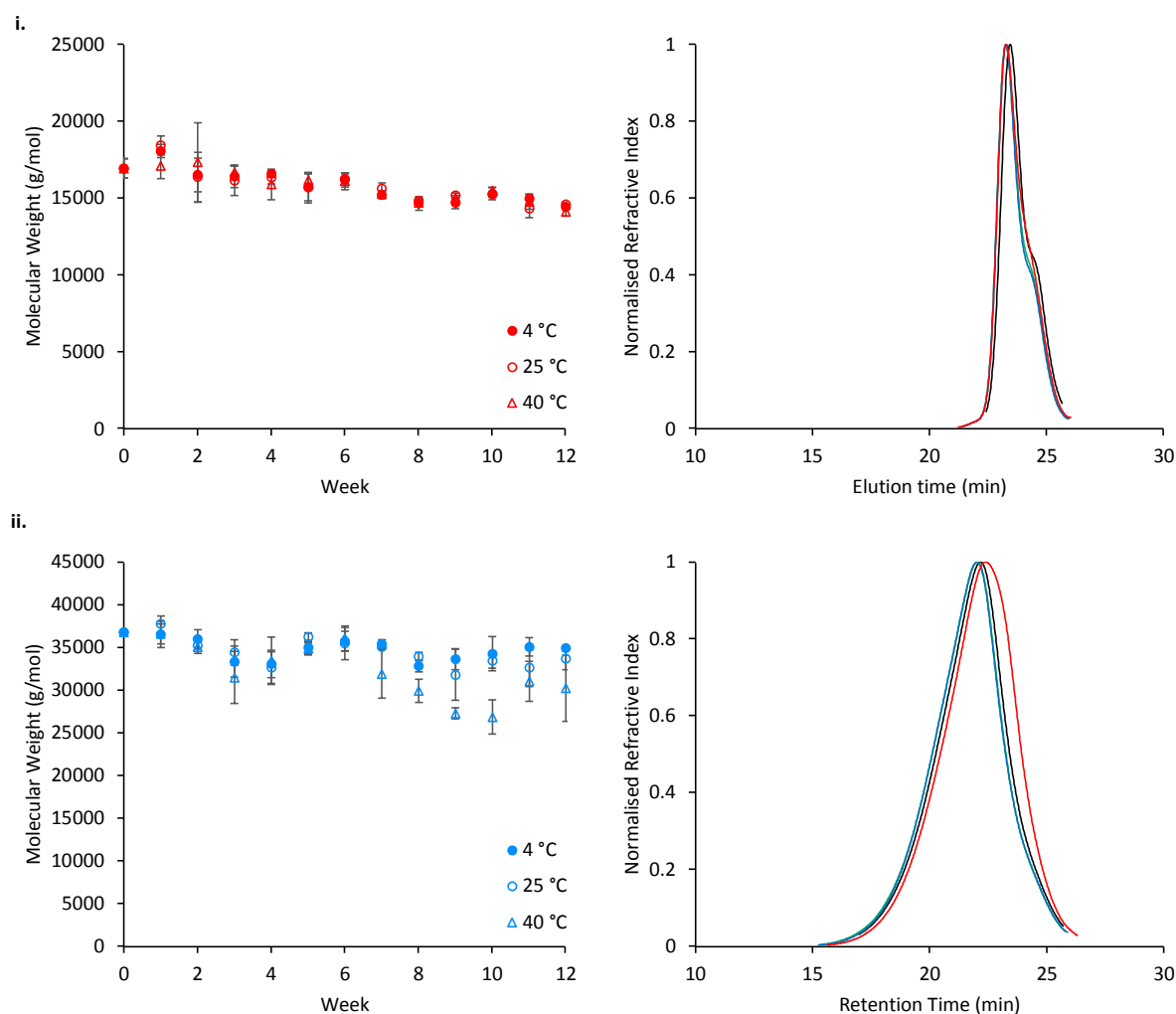
Figure 11. Stability of poloxamer 407 (i) and PNIPAM 98 -PEG 122 -PNIPAM 98 (ii) at 4, 25 and 40 °C. Variation in the number-average molecular weight is shown on the left. GPC traces are shown on the right, with week 0 shown in black, and week 12 at 4, 25 and 40 °C shown in green, blue and red, respectively.
