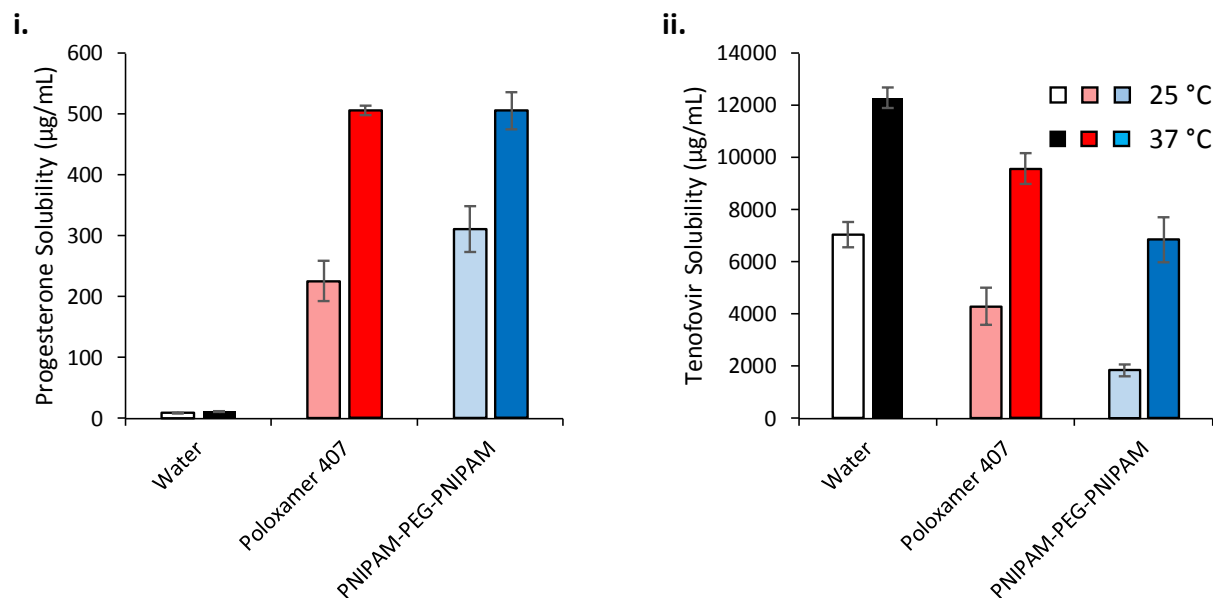
Figure 9. Saturation solubility of progesterone (i) and tenofovir disoproxil fumarate (ii) in 20 % (w/v) poloxamer 407 (red) and 50 % (w/v) PNIPAM 98 -PEG 122 -PNIPAM 98 (blue) at 25 and 37 °C (light and dark colours, respectively).
