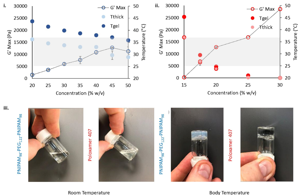
Figure 3. Tthick (light circle), Tgel (dark circle), and G'max (hollow circle with dashes) as a function of concentration for PNIPAM 98 -PEG 122 -PNIPAM 98 (i, blue) and poloxamer 407 (ii, red). The temperature range which would allow for in situ thickening of polymer solutions is overlaid in grey. Please note that Tthick and Tgel are omitted for 30 % (w/v) poloxamer 407 as they were not present in the rheogram. Data presented as mean \pm standard deviation, n = 3. Images of the thermoversible gelators are included (iii) at room temperature and body temperature, 37 °C.
