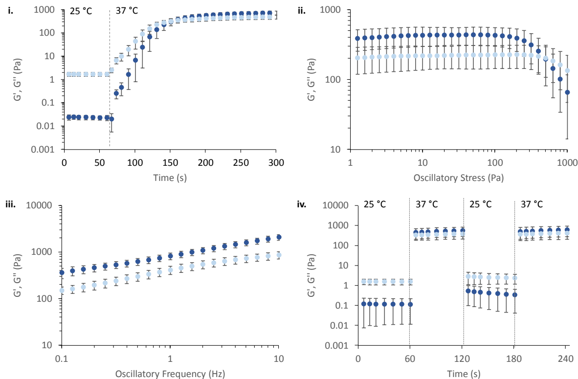
Figure 4. (i) Determination of gelation time for PNIPAM 98 -PEG 122 -PNIPAM 98 (50 % (w/v)). (ii) Oscillatory stress sweep of PNIPAM 98 -PEG 122 -PNIPAM 98 (50 % (w/v)), and (iii) oscillatory frequency sweep. (iv) thermal cycling of PNIPAM 98 -PEG 122 -PNIPAM 98 (50 % (w/v)) to demonstrate reversibility of the gelation process. G' and G'' are shown as dark and light blue markers, respectively. Data presented as mean \pm standard deviation, n = 3 .
