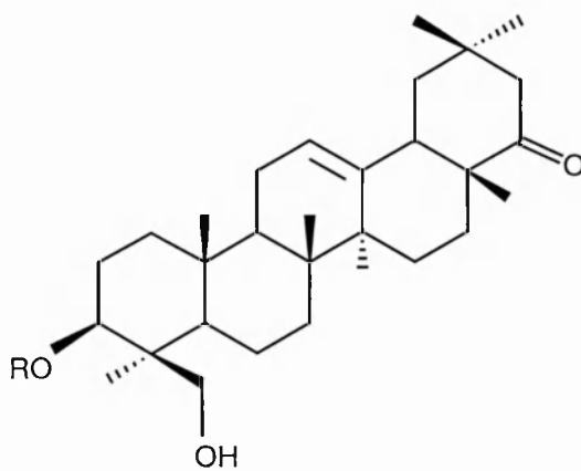
FIGURE 1.6. Structures of group E saponins.
