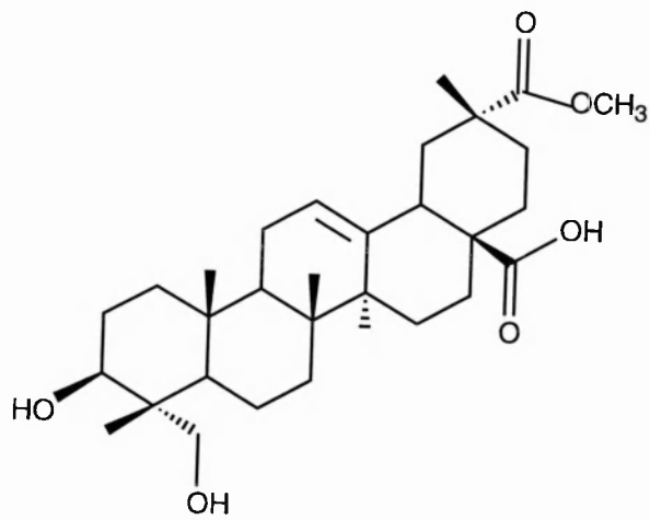
FIGURE 1.9. Structure of phytolaccagenic acid.
