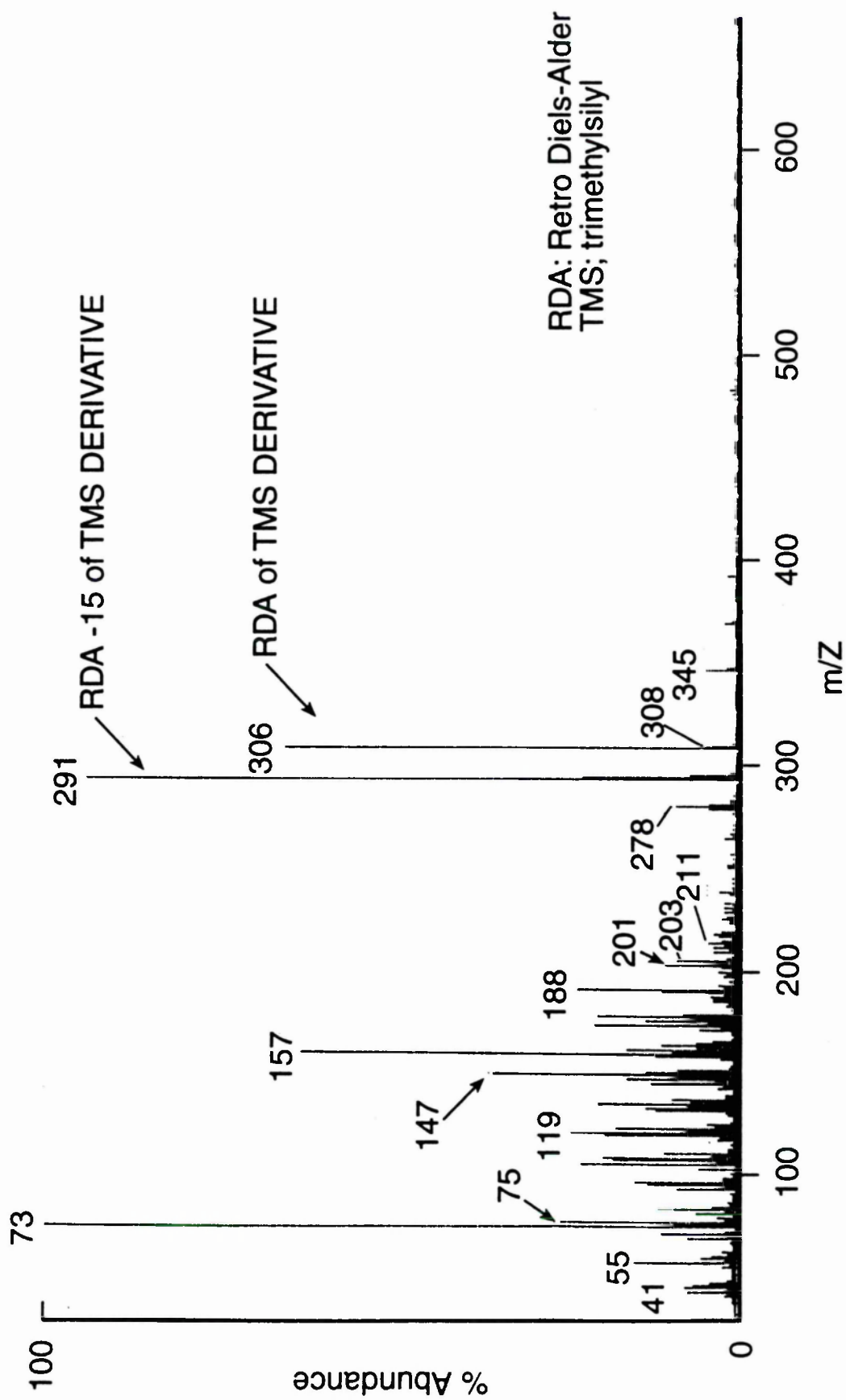
FIGURE 4.6 GC mass spectrum of the saponin derived from the novel saponin.
