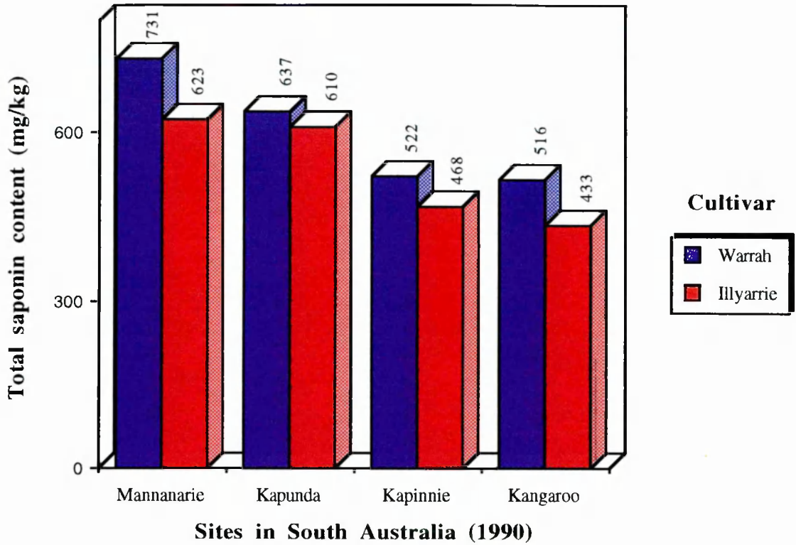
FIGURE 2.6. Effect of cultivar and location (site within a region) on the total saponin content (mg/kg) of L. angustifolius in the 1990 growing year.
