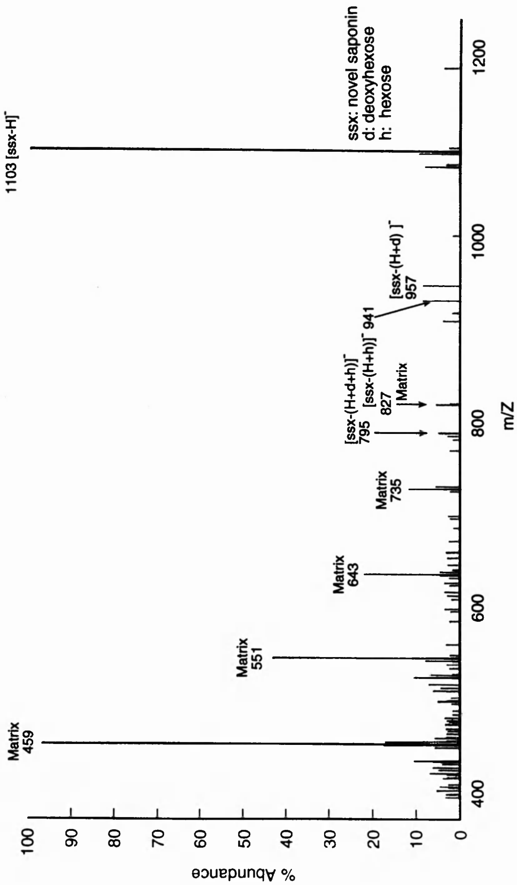
FIGURE 4.3 FAB mass spectrum in the negative mode of the novel saponin.
