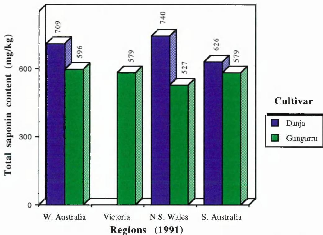
FIGURE 2.5. Effect of cultivar and location (region) on the total saponin content (mg/kg) of L. angustifolius in the 1991 growing year.
