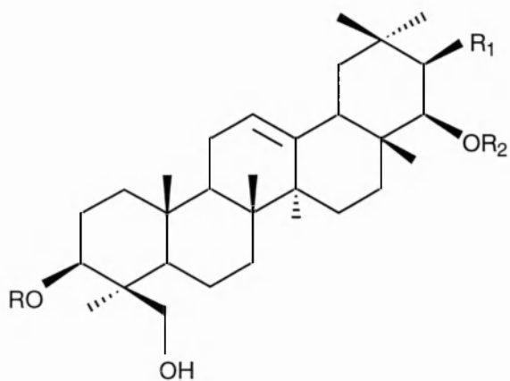
FIGURE 1.5. Structures of group A and B saponins.
