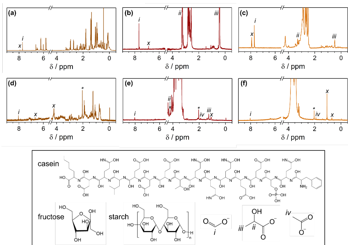
Figure 3. ^1\text{H-NMR} spectroscopy of (a) casein, (b) fructose and (c) starch after photoreforming with CdS/CdO x QDs in 10 M NaOD; and (d) casein, (e) fructose and (f) starch after photoreforming with ^{\text{H}_2\text{N}^{15}\text{CN}_x|\text{Ni}_2\text{P}} in D 2 O. (g) Chemical structures of casein, fructose, starch, formate, lactate and acetate, and their peak assignments. (x) are unassigned oxidation products, (*) are trace amounts of acetone in contamination, and unlabelled peaks are from the substrate structure. Photoreforming conditions: CdS/CdO x QDs (0.5 nmol) in NaOD (10 M) in D 2 O (1 mL) or ^{\text{H}_2\text{N}^{15}\text{CN}_x|\text{Ni}_2\text{P}} (1.5 mg mL -1 ) in D 2 O (1 mL), pre-treated substrate (25 mg mL -1 ), simulated solar light (4 days, AM 1.5G, 100 mW cm -2 , 25 °C).
