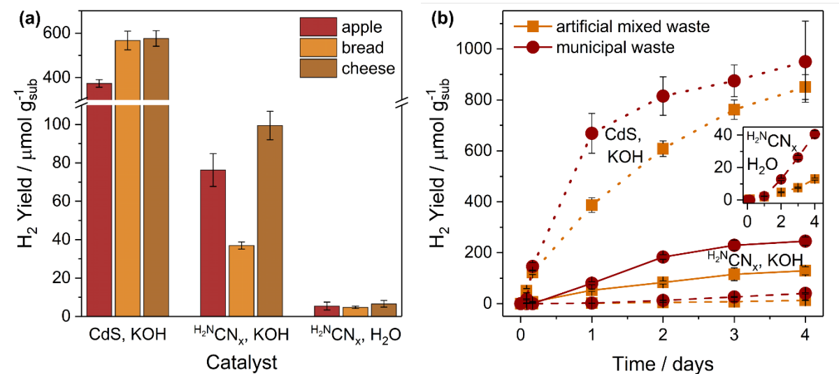
Figure 4. Photoreforming of real-world waste, including (a) apple, bread and cheese, and (b) artificial mixed and municipal wastes; inset shows the bottom two traces ( ^{\text{H}_2\text{N CN}_x|\text{Ni}_2\text{P} in \text{H}_2\text{O} ) in more detail. Artificial mixed waste consists of 5 \text{ mg mL}^{-1} each of apple, bread, cheese, cardboard and polyethylene terephthalate bottle. Conditions: CdS/CdO x QDs ( 1 \text{ nmol} ) in 10 \text{ M aq. KOH} ( 2 \text{ mL} ) or ^{\text{H}_2\text{N CN}_x|\text{Ni}_2\text{P}} ( 1.5 \text{ mg mL}^{-1} ) in either 10 \text{ M aq. KOH} ( 2 \text{ mL} ) or \text{H}_2\text{O} ( 2 \text{ mL} ); pre-treated substrate ( 25 \text{ mg mL}^{-1} apple, bread, cheese or artificial mixed waste or 12.5 \text{ mg mL}^{-1} municipal waste); simulated solar light ( 20 \text{ h} for a, 4 days for b, AM 1.5G, 100 \text{ mW cm}^{-2} , 25 \text{ }^\circ\text{C} ).
