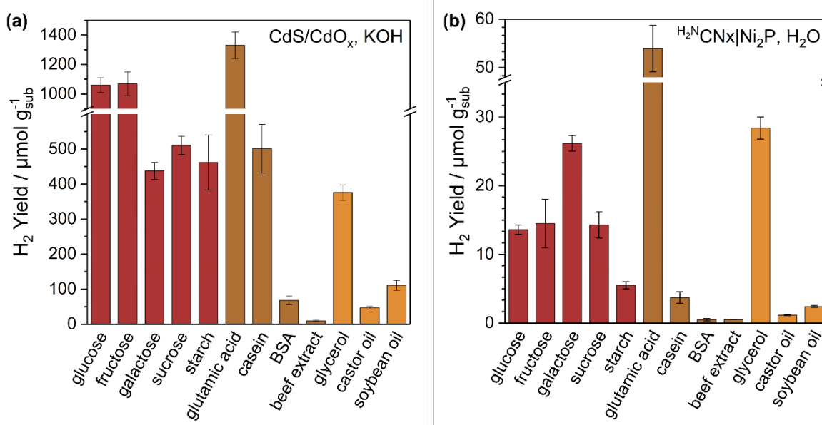
Figure 2. Photoreforming of food-derived molecules with (a) CdS/CdO x QDs in alkaline solution and (b) H 2 N CN x |Ni 2 P in H 2 O. Conditions: CdS/CdO x QDs (1 nmol) in 10 M aq. KOH (2 mL) or H 2 N CN x |Ni 2 P (1.5 mg mL -1 ) in H 2 O (2 mL); substrate (25 mg mL -1 ) pre-treated (24 h with stirring) in 10 M KOH at 40 °C for a or H 2 O at 80 °C for b; simulated solar light (20 h, AM 1.5G, 100 mW cm -2 , 25 °C).
