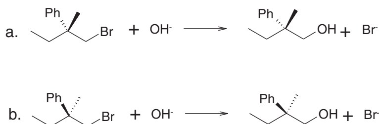
Figure 4 Short RInChIKeys, version B, for a pair of enantiomeric reactions. a. Short RInChIKey = bSA-BEANN-CPQZBLWAMR-DVCHMHGSMQ-EANNATPGMB-MILF-MCLVE-NEANN. b. Short RInChIKey = bSA-BEANN-CPQZBLWAMR-DVCHMHGSMQ-EANNATPGMB-MDSDX-MDUXS-NEANN.
