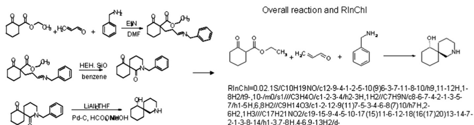
Figure 9 Generation of a RInChI for an overall reaction (multistep reaction).
