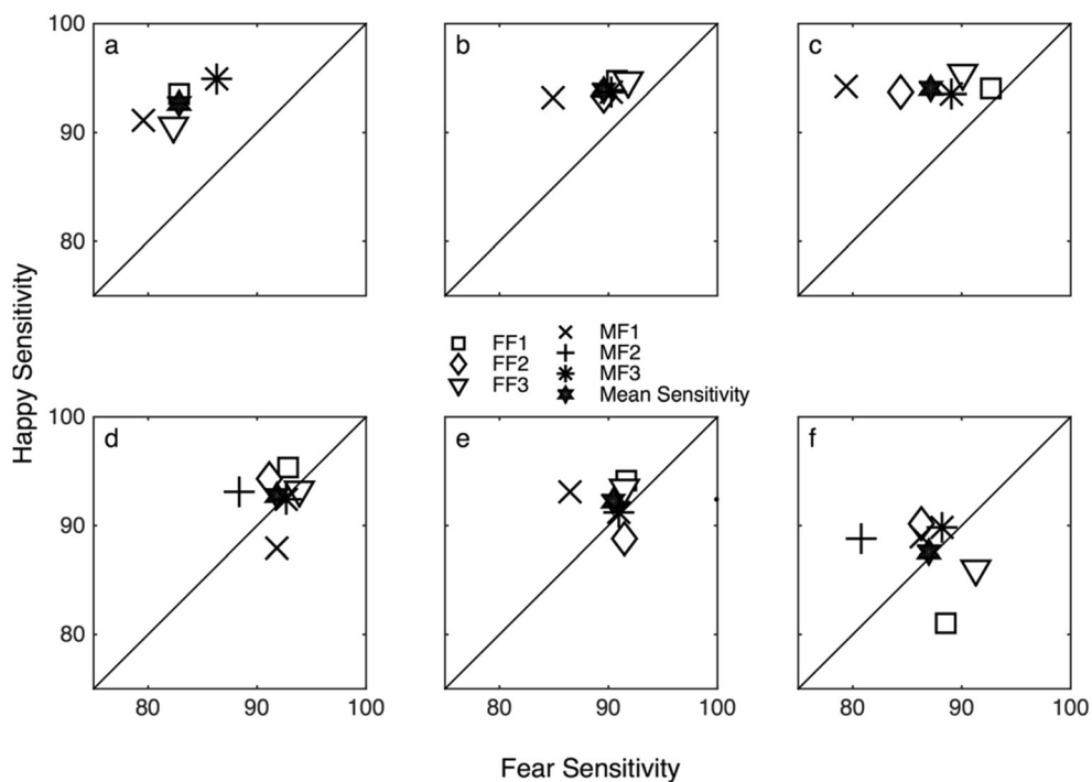
Fig. 7 Sensitivity to happy (y-axis) and fearful (x-axis) expressions for six individual participants (a–f) for each unique face (three female [FF] and three male [MF] faces; see Fig. 2). Mean sensitivity is represented by a filled star. Figure 6b is replotted here as in Fig. 7a. All other details as in Fig. 3
