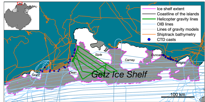
Figure 1. The geographic location and data coverage of Getz. The blue area is ocean. The gray area is Getz Ice Shelf. The white area is grounded ice. Colored lines and marks denote the ice shelf extent (Mouginot et al., 2017), helicopter gravity data, NASA OIB data (Cochran and Bell, 2010a), ship track bathymetry (Nitsche et al., 2007) and CTD casts (Locarnini et al., 2013). This plot is generated from the Antarctic Mapping Tool (Greene et al., 2017).
