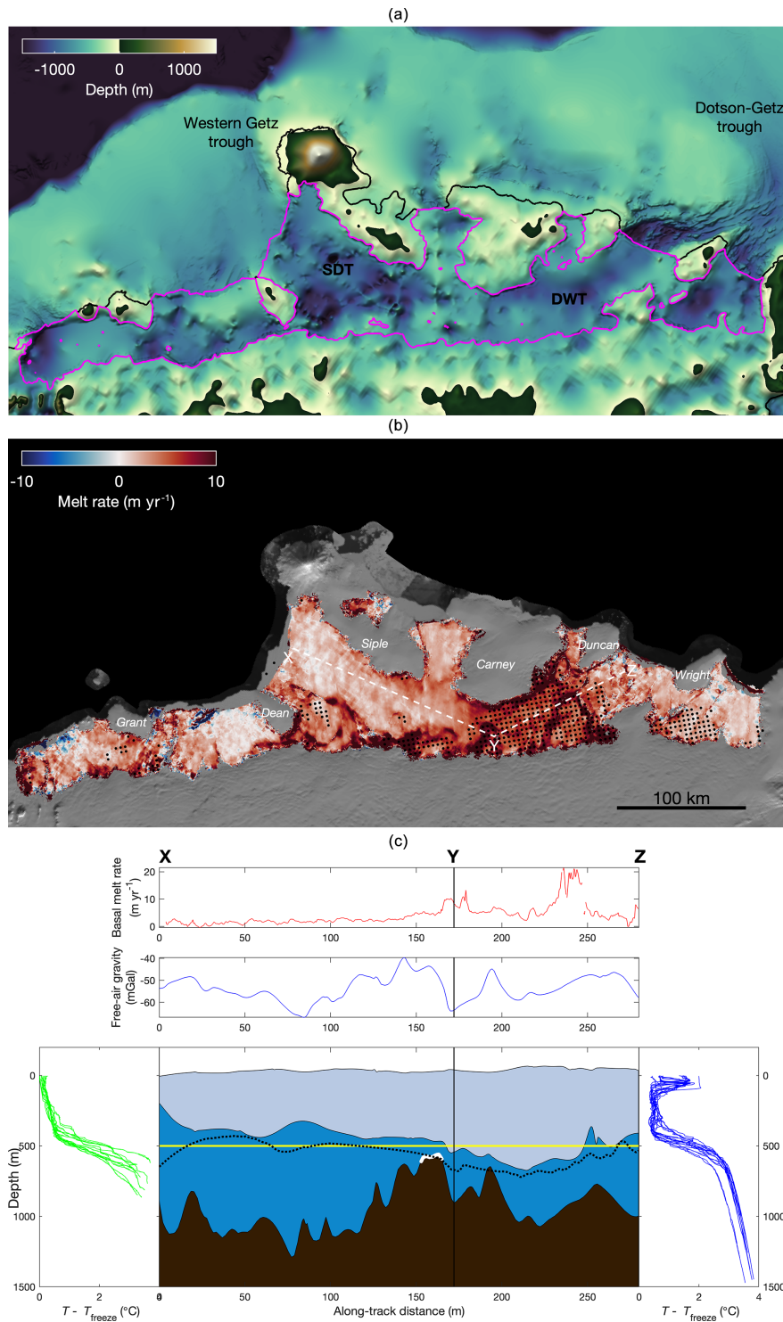
Figure 2. The shape of the seafloor, basal melt rates, and along-profile view of the study area. (a) The bathymetry of the Getz Ice Shelf. The profile XYZ crosses the trough between Dean Island and Siple Island, the bathymetric sill, and the trough between Duncan and Wright Islands. The purple is the ice shelf outline (Mouginot et al., 2017). The bathymetry of the continental shelf is from IBCSO (Arndt et al., 2013). (b) The observed basal melt rate. Black stippling indicates ice bottom elevations that are below the 500 m depth of the thermocline. The background is the MODIS-derived Mosaic of Antarctica (MOA; Scambos et al., 2007). (c) Upper panel shows the basal melt rate along profile XYZ. The lower panel shows the elevations of ice and bedrock along profile XYZ, with the depth-temperature profiles from western and eastern Getz. Ocean is blue; ice is light blue, and the bedrock is brown. The white indicates the location of the bathymetric sill. The dashed black line is the bathymetry from Bedmap2 (Fretwell et al., 2013). The horizontal yellow line indicates the mean thermocline depth. The thermal forcing T - T_{\text{freeze}} is calculated from CTD casts (Locarnini et al., 2013).
