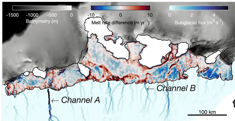
Figure 3. The melt rate difference between observed melt rate and melt rate with no discharge. Red indicates regions where observed melt rates are higher than can be explained by temperature- and depth-dependent forcing alone. The blue fluxes indicate subglacial meltwater. The gray background is the bathymetry from IBCSO (Arndt et al., 2013).
