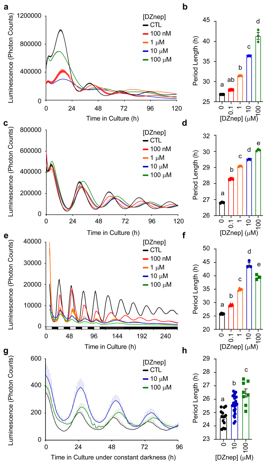
Fig. 2 Circadian rhythms are a quantitative gauge for methylation deficiency in Metazoa. a Mean luminescence ± SEM of human Bmal1-luc U-2 OS cells 25 treated with increasing concentrations of DZnep; b shows mean ± SEM of period, n = 3 dishes. c Mean luminescence ± SEM of PER2::LUC MEF 24 treated with DZnep, n = 3 dishes; mean ± SEM of period shown in d . e Mean luminescence ± SEM of Per1b-luciferase PAC-2 zebrafish cells treated with DZnep, n = 4 dishes; mean ± SEM of period shown in f ; note the initial 96 h of data performed under light/dark cycles. g Mean luminescence ± SEM of ptim-TIM-LUC Drosophila halteres treated with DZnep, n = 8 independent halteres, with only the upper segment of the error bars shown for clarity; mean ± SEM of period shown in h . All bar graphs analyzed by One-Way ANOVA followed by Bonferroni's test; all indicated comparisons ( a vs. b vs. c vs. d vs. e ), at least p < 0.05 .
