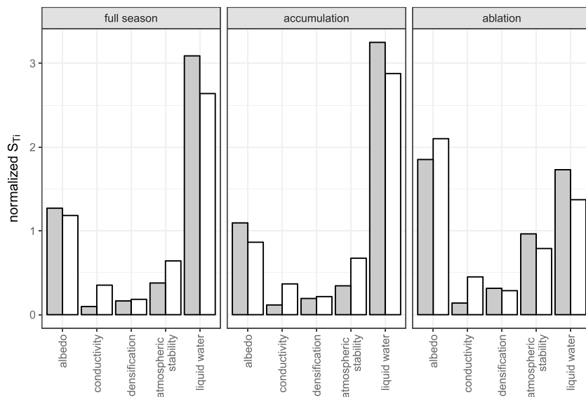
Figure 12. Mean interannual total-order sensitivity indices resulting from two different SA strategies normalized by its mean S_{T_i} value. (gray bars) Perturbing the shown parameters during the sensitivity analysis with no forcing error and the default model parametrization. (white bars) Following the workflow presented in section 2.5 including perturbations of forcing errors and model parametrization.
