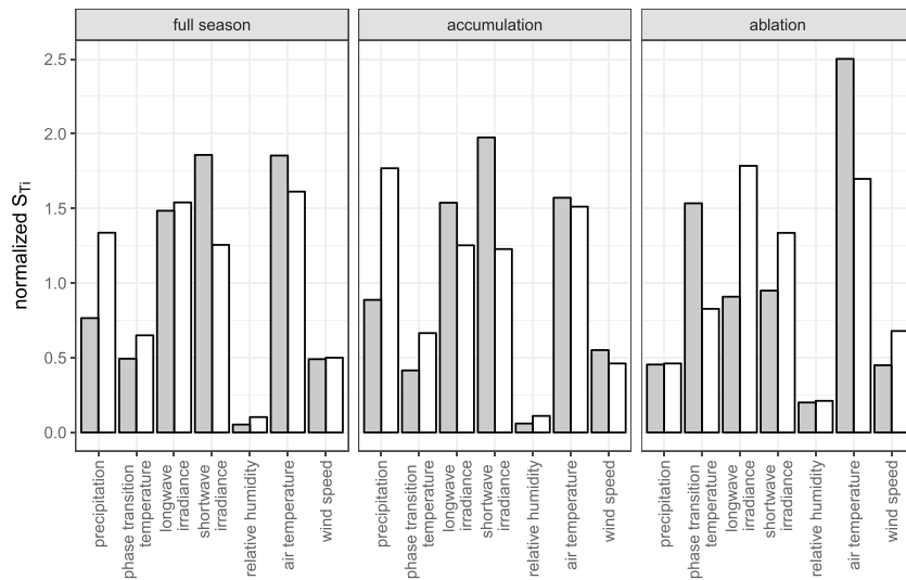
Figure 11. Mean interannual total-order sensitivity indices resulting from two different sensitivity analysis strategies normalized by its mean S_{T_i} value. (gray bars) Perturbing the shown parameters during the sensitivity analysis for just one snow model option (Factorial Snowpack Model configuration 0) and its default parametrization. (white bars) Following the workflow presented in section 2.5 including perturbations of model structure and parametrization.
