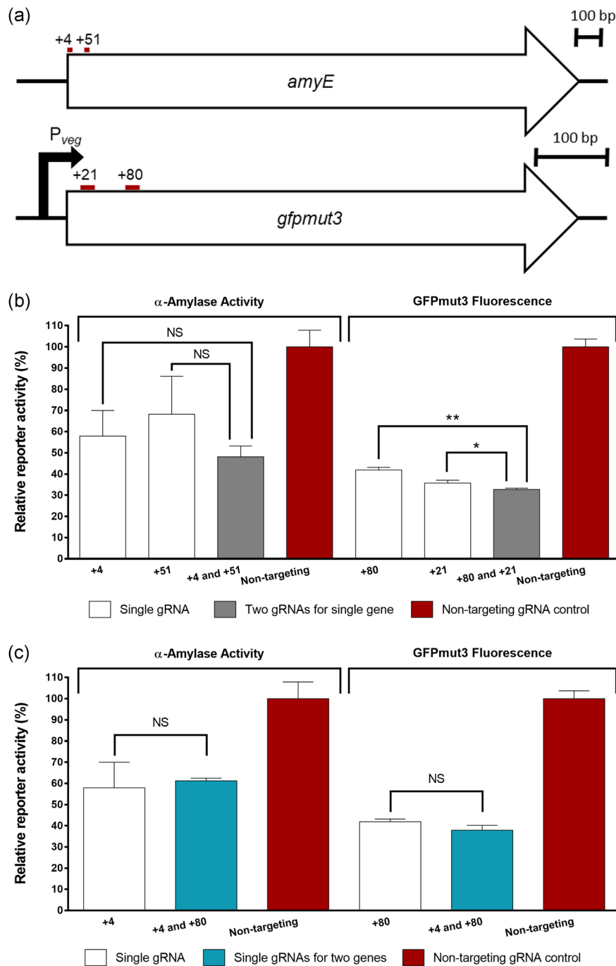
FIGURE 4 Relative \alpha -amylase activity and GFPmut3 fluorescence following dMAD7-mediated multiplexing CRISPRi in BAC0288. (a) Schematic diagrams of gRNA binding sites for dMAD7 within amyE and gfpmut3 . Values represent the distance of each targeted PAM site from the start codon on the non-template DNA strand. (b) Investigation for an additive multiplexed CRISPRi effect when two gRNAs target a single gene. (c) Investigation for a multiplexed CRISPRi effect when two gRNAs target different genes within the same strain. Bars represent extracellular \alpha -amylase activity, or GFPmut3 fluorescence intensity, normalized by OD 600 nm , relative to the nontargeting gRNA control strain, after 24 hr of growth. The horizontal axis indicates the targeted PAM site(s) distance to the amyE or gfpmut3 start codon (Strains used: +4: BAC0381; +51: BAC0382; +4 and +51: BAC0377; +4 and +80: BAC0378; +80: BAC0368; +21: BAC0351; +80 and +21: BAC0380). White bars indicate strains in which a single gRNA is utilized to target a single gene. Gray bars indicate strains in which the effect of two gRNAs on a single gene is investigated. Blue bars indicate BAC0378 in which the effect of single gRNAs on two different genes is investigated. Red bars indicate the negative control strain, BAC0350, in which a nontargeting gRNA is expressed alongside dMAD7. Error bars indicate the standard deviation between three biological replicates. * p < .05 ; ** p < .01 . Two-tailed p values were derived following unpaired t test with Welch's correction. gRNA, guide RNA; NS, not significant [Color figure can be viewed at wileyonlinelibrary.com ]
