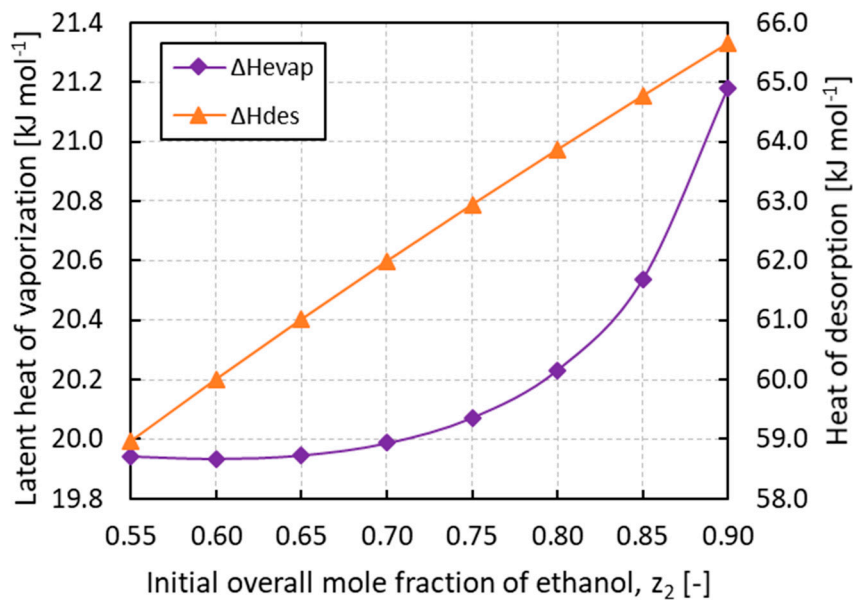
Figure 8. Latent heat of vaporization ( \Delta H_{evap} ) and heat of desorption ( \Delta H_{des} ) of ammonia/ethanol mixture vs. the initial overall mole fraction of ethanol z_2 .
