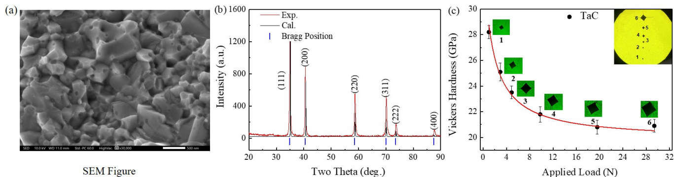
Figure 1 (a) SEM micrograph of TaC sample synthesised at 5.5 GPa and 1400 °C. (b) X-ray diffraction pattern ( \lambda = 1.5404 \text{ \AA} ) of recovered TaC sample. Calculated XRD pattern for lattice constant a = 4.455 \text{ \AA} . (c) Vickers hardness ( H_v ) test results of TaC for applied loads from 0.98 N to 29.4 N. The insert displays the Vickers indentation impression at different loading force. The red line is an asymptotic fit to the data with the following relation: H_v = 19.8 \times \exp(1.2/(F+2.1)) , where F is the load (N). The asymptotic measured hardness value is 20.9 GPa for TaC.
