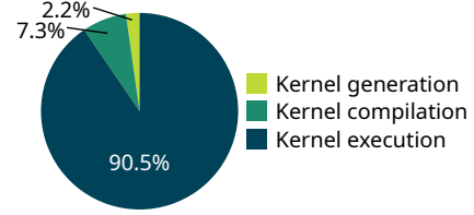
Figure 2. Time breakdown for the LIFT exploration process. Kernel generation includes time to rewrite and compile LIFT expressions to OpenCL kernels. Kernel compilation is the vendor-provided OpenCL compiler time. Kernel execution is the time required to execute all generated kernels.
