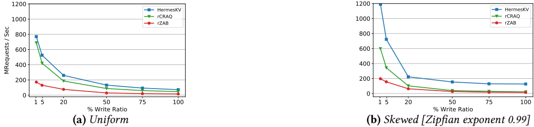
Figure 5. Throughput for 1% to 100% write ratio. [5 nodes]
