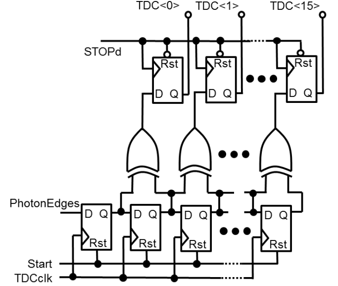
Fig. 8. 16-bin clocked shift-register multi-event TDC (METDC).
