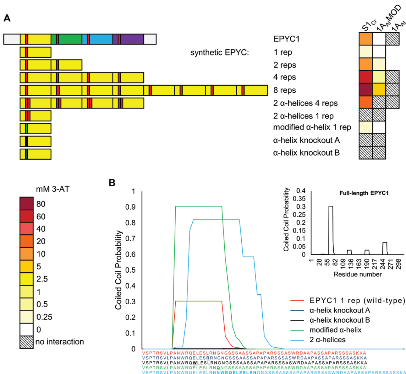
Fig. 4. EPYC1 can be modified to increase the interaction strength with SSUs. (A) Synthetic variants of EPYC1 are based on the first repeat regions (yellow) and the predicted α-helix (red). The heat map indicates interaction strength measured with yeast two-hybrid assays by the capacity for growth on increasing concentrations of 3-AT (mM). See Supplementary Fig. S3D for raw Y2H image data. (B) Predicted coiled-coil domain strengths for synthetic variants of the first repeat region of EPYC1 using the PCOILS bioinformatic tool. Matching colour-coded amino acid sequences are shown below, with residues that differ from the wild-type sequence shown in bold. The inset shows the prediction for full-length EPYC1.
