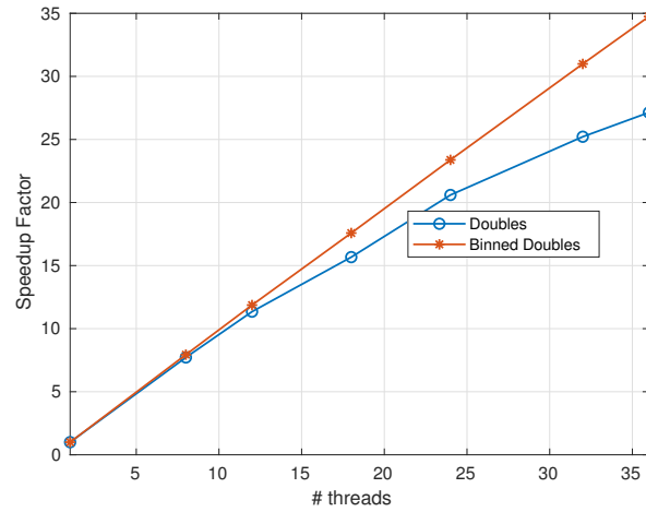
Fig. 3. Comparison of speedup factor of Conjugate Gradient solver for built-in doubles and binned doubles with K = 3 on Cirrus.
