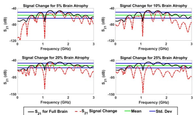
Fig. 7. Simulation plots showing changes in transmission coefficient ( S_{21} ) between a normal brain and brain with 5%, 10%, 20%, and 25% brain atrophy.
