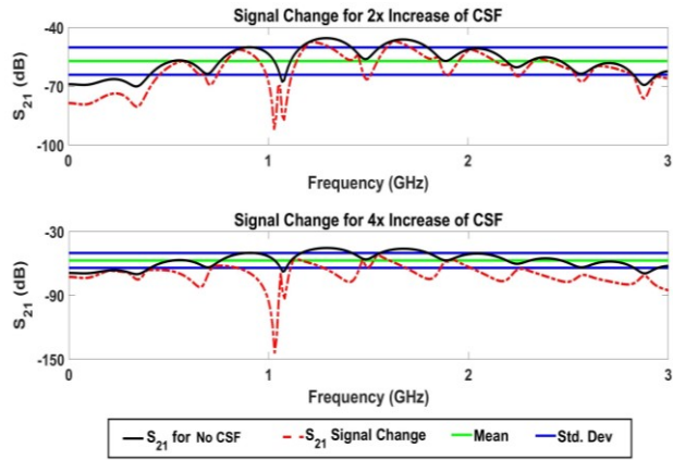
Fig. 9. Simulation plots showing changes in S_{21} between a brain with normal CSF levels and brain with 2x and 4x CSF levels in the lateral ventricles.
