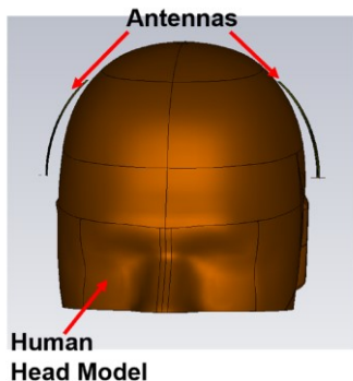
Fig. 2. Human head CST model and antennas that were used for simulations of brain atrophy and lateral ventricle enlargement.
