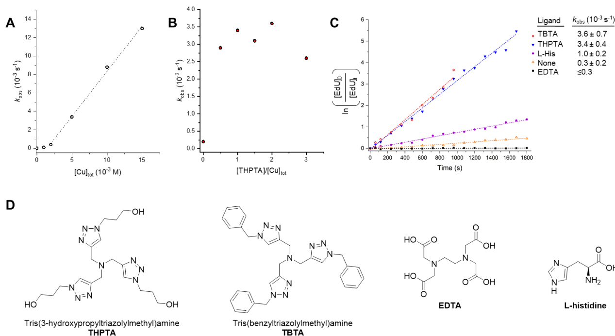
Figure 5: Investigating catalyst composition effects on the kinetics of the CuAAC reaction between EdU and biotin-PEG3-azide in DMSO/H 2 O 3:2 v/v. A Plot of k_{obs} as a function of [Cu]_{tot} , showing a first-order dependence on [Cu]_{tot} . A linear fitting is only applied between [Cu]_{tot} = 2 - 15 mM, due to the suspected presence of low concentrations of inhibitors in the reactants. Experimental conditions described in Entry 1, Table 1. Tabulated data with k_{obs} \pm 0.5 RMSE see Table S1. B Plot of k_{obs} as a function of [Cu]/THPTA ratio. Experimental conditions described in Entry 2, Table 1. Tabulated data with k_{obs} \pm 0.5 RMSE see Table S2. C Plot of CuAAC reaction with different CuAAC ligands with k_{obs} \pm 0.5 RMSE. Experimental conditions described in Entry 3, Table 1. D Chemical structure of the Cu(I) ligands, THPTA, TBTA, EDTA and L-Histidine.
