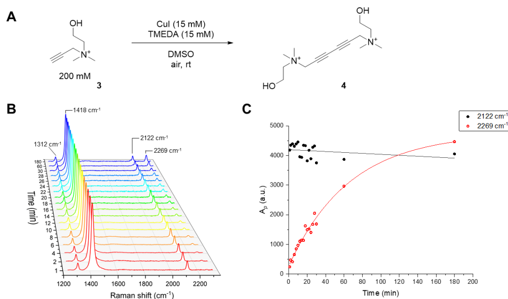
Figure 6: Reaction monitoring of the Glaser-Hay homocoupling of propargyl choline using Raman spectroscopy. A Glaser-Hay reaction of propargyl choline (200 mM) using CuI (15 mM, 7.5 mol%) and TMEDA (15 mM, 7.5 mol%) in DMSO. B Raman spectra of the reaction mixture in A acquired at the indicated timepoints following addition of the Cu/TMEDA catalyst. An aliquot of the reaction mixture was removed at each timepoint and the individual Raman spectra presented between 0-180 min. Spectra were acquired using \lambda_{\text{ex}} = 532 nm for 20 s using a 20 \times objective lens. The Raman spectra were normalised to the intensity of the peak at 1418 \text{cm}^{-1} (DMSO CH def.). C Integration analysis of the Raman peaks at 2122 \text{cm}^{-1} (propargyl choline) and 2269 \text{cm}^{-1} (dimer) presented in B . A_i = peak area @ 2122 \text{cm}^{-1} / 2269 \text{cm}^{-1} . The lines through the data are merely a guide to the eye, not kinetic fitting.
