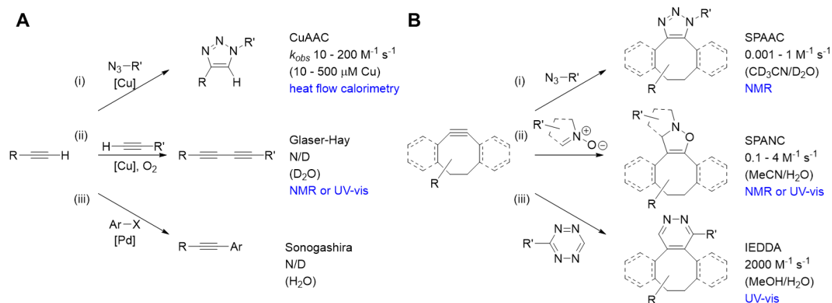
Figure 1: Bioorthogonal reactions of terminal alkynes ( A ) and strained alkynes ( B ), with approximate rate constants in aqueous based media (N/D = not determined). A (i) copper(I) catalysed azide alkyne cycloaddition (CuAAC); [23] (ii) Glaser-Hay reaction; [24] (iii) Copper-free Sonogashira reaction; [25] B (i) strain-promoted azide alkyne cycloaddition (SPAAC); [26] (ii) strain-promoted alkyne nitron cycloaddition (SPANC); [26] (iii) Inverse electron demand Diels-Alder (IEDDA). [27]
