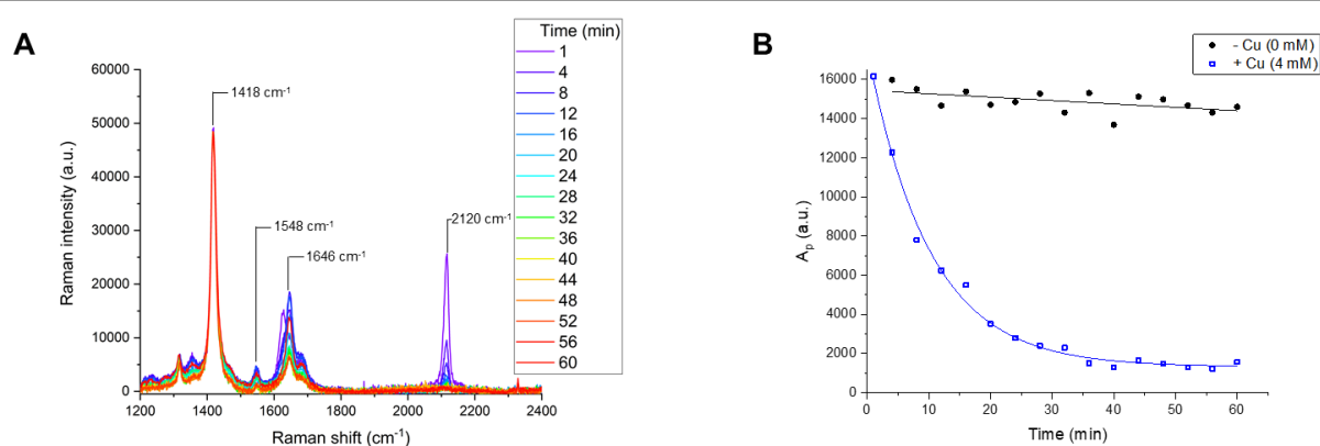
Figure 4: Reaction monitoring of the CuAAC reaction between EdU ( 1 ) and biotin-PEG3-azide ( 2 ) using Raman spectroscopy. A Raman spectra of reaction mixture comprising EdU (50 mM), biotin-PEG3-azide (50 mM), \text{CuSO}_4 (4 mM) and ascorbic acid (20 mM) in \text{DMSO}(\text{aq.}) . An aliquot of the reaction mixture was removed at each timepoint and the individual Raman spectra presented between 0-60 min. Spectra were acquired using \lambda_{\text{exc}} = 532 nm for 20 s using a 20 \times objective lens. The Raman spectra were normalised to the intensity of the peak at 1418 \text{cm}^{-1} (DMSO CH def.). B Integration analysis of the normalised Raman peak at 2120 \text{cm}^{-1} ( \text{C}\equiv\text{C} , EdU) for the reaction presented in A (blue squares, +Cu (4 mM) with exponential fitting applied) and a control reaction (black circles, -Cu, linear fitting) where [\text{Cu}] = 0 mM. A_p = peak area @ 2120 \text{cm}^{-1} .
