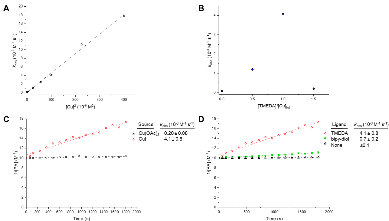
Figure 7: Empirical correlations for the kinetics of the Glaser-Hay homocoupling of phenylacetylene (PA). Experimental conditions tabulated in Table S3. A Correlation of the observed second-order rate constant with total [Cu]. Experimental conditions described in Entry 1, Table S3. Tabulated data with k_{\text{obs}} \pm 0.5 RMSE see Table S4. B Effect of Cu:TMEDA ratio on observed second-order rate constant. Experimental conditions described in Entry 2, Table S3. Tabulated data with k_{\text{obs}} \pm 0.5 RMSE see Table S5. Empirical second-order kinetic analysis of Glaser-Hay reactions with various Cu-sources ( C ), and ligand ( D ) with k_{\text{obs}} \pm 0.5 RMSE. Experimental conditions described in Entries 3 and 4, Table S3.
