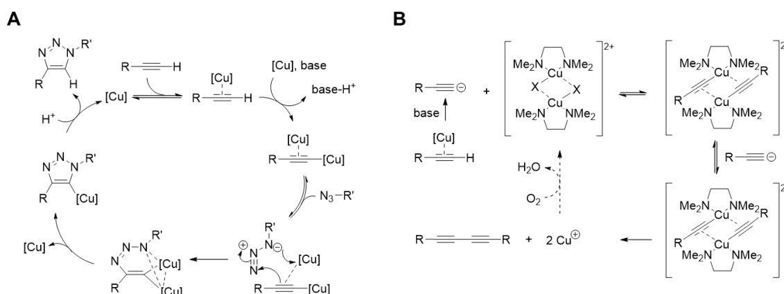
Figure 2: Simplified mechanisms for the catalytic cycle of (A) the CuAAC reaction; [29a] (B) the Glaser-Hay reaction. [34]
