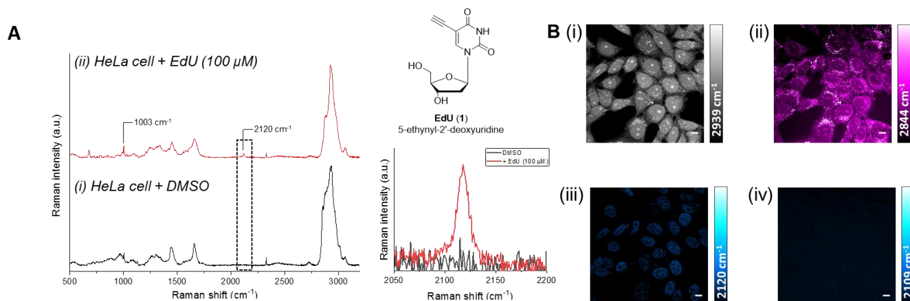
Figure 3: Detection of alkyne-labelled DNA using EdU ( 1 ) and Raman imaging. A Spontaneous Raman spectroscopy of single fixed HeLa cells treated with (i) DMSO and (ii) EdU (100 \mu\text{M} , 18 h). [18] The spectra were normalised to the intensity of the peak at 1003 \text{cm}^{-1} (phenylalanine ring breathing mode), scaled between -1000 – 20000 counts and offset for clarity. Peak annotations: 1003 \text{cm}^{-1} (phenylalanine ring breathing mode); 2120 \text{cm}^{-1} ( \text{C}\equiv\text{C} , EdU). Raman spectra acquired using \lambda_{\text{ex}} = 532 nm using a 50 \times objective lens and 30s integration time. Inset: chemical structure of EdU (top) and expansion of the EdU alkyne region (2050 – 2220 \text{cm}^{-1} indicated by the dashed box; bottom). B SRS imaging of HeLa cells treated with EdU (100 \mu\text{M} , 18 h). [18] SRS images were acquired at (i) 2939 \text{cm}^{-1} ( \text{CH}_3 ), (ii) 2844 \text{cm}^{-1} ( \text{CH}_2 ), (iii) 2120 \text{cm}^{-1} ( \text{C}\equiv\text{C} ), (iv) 2109 \text{cm}^{-1} ( \text{C}\equiv\text{C} ).
