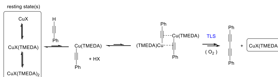
Figure 8: Mechanism for the Glaser-Hay reaction consistent with kinetic data obtained by Raman spectral analysis. TLS = turnover rate-limiting step.
