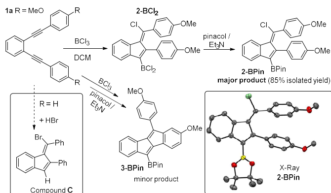
Figure 1: The functionalisation of 1a using \text{BCl}_3 and subsequent pinacol protection. Inset right, solid state structure of 2-BPin , ellipsoids at the 50% probability level and hydrogens omitted for clarity. Inset left, previous work cyclising with \text{HBr} .
