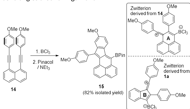
Figure 4: Borylative cyclisation of 14 . Inset right, the zwitterionic vinyl cations derived from 1a and 14 on combination with BCl 3 .
