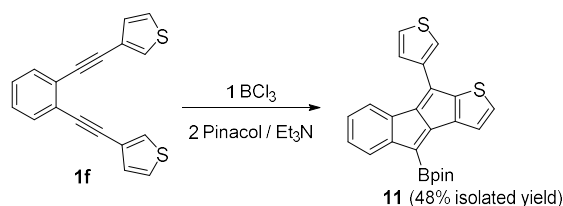
Scheme 5: Borylative cyclisation of diyne 1f .
