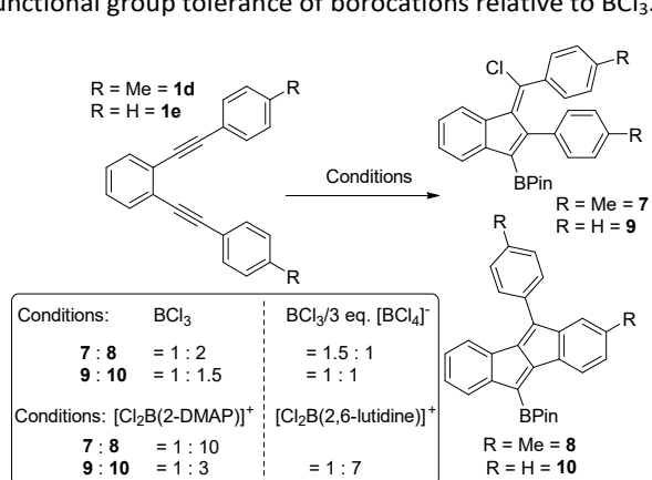
Scheme 4: Change in product ratio on altering the boron electrophile or by the addition of an exogenous chloride source.
