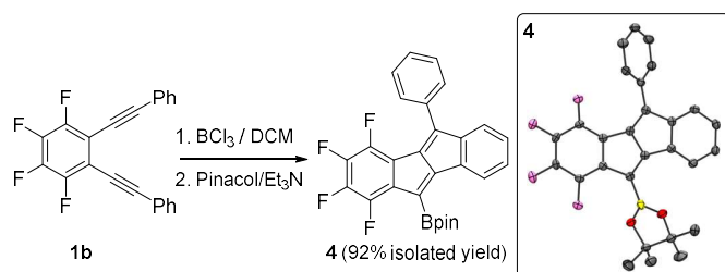
Figure 2: Borylative cyclisation of 1b . Inset right, the solid state structure of 4 , ellipsoids at 50% probability level and hydrogens omitted for clarity.
