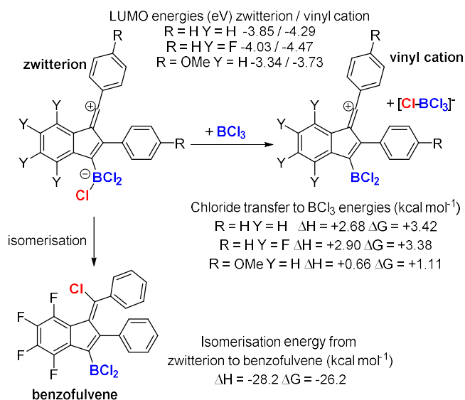
Scheme 2: Calculations of the energy change in chloride transfer reactions (all at the M06-2x/6-311G(d,p) / PCM (DCM) level. In the vinyl cation the anion and cation were calculated at infinite distance.
