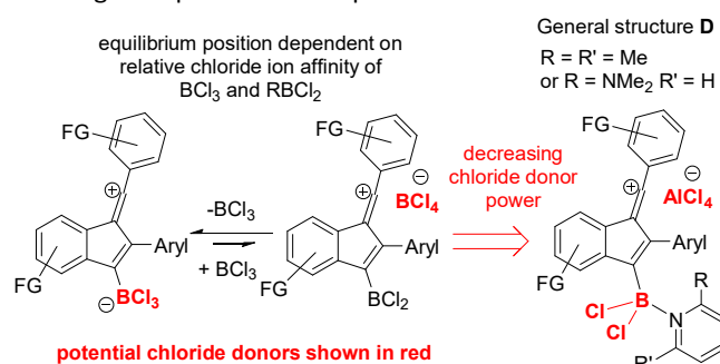
Figure 3: Potential sources of chloride during the borylative cyclisation of diynes 1x using different boron electrophiles.
