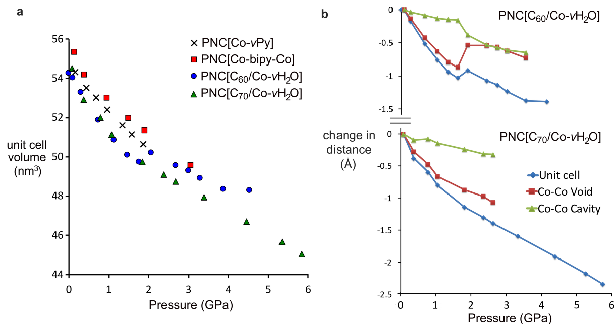
Figure 2. Pressure-induced changes in crystal structure. (a) Change in unit cell volume on increasing pressure for PNC[Co- \nu Py], PNC[Co-cbipy-Co], PNC[ c C 60 /Co- \nu H 2 O] and PNC[ c C 70 /Co- \nu H 2 O]. (b) Change in Co-to-Co distances both across the void and fullerene-containing cavity within PNC[ c C 60 /Co- \nu H 2 O] and PNC[ c C 70 /Co- \nu H 2 O].
