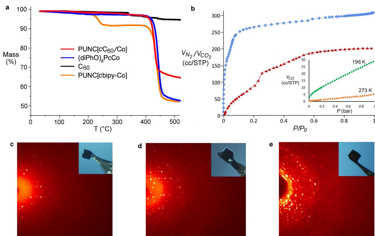
Fig. 4. Thermal, gas adsorption and XRD data supporting the stability of PUNC[ c C 60 /Co]. (a) Thermal gravimetric analysis of PUNC[ c C 60 /Co], PUNC[Co- c bipy-Co], (diPhO) 8 PcCo and C 60 demonstrating the greater thermal stability of PUNC[ c C 60 /Co] relative to PUNC[Co- c bipy-Co], with the latter losing its bipy ligand at ~200 °C. (b) Adsorption isotherms of PUNC[ c C 60 /Co] outgassed under vacuum at 125 °C for 2h: for N 2 (◆) at 77 K, CO 2 (▲) at 196 K and (inset) CO at 196 K (●) and 273 K (○), (desorption data follows closely that of adsorption). (c-f) Diffraction images of a single-crystal (micrograph inset) of PUNC[ c C 60 /Co] after soaking in (c) boiling water for 24 h; (d) boiling aqueous 2M NaOH for 24 h; and (e) boiling aqueous 2M HCl for 24 h (note that broadening of the diffraction spots is ascribed to fracture of the crystal rather than loss of order).
