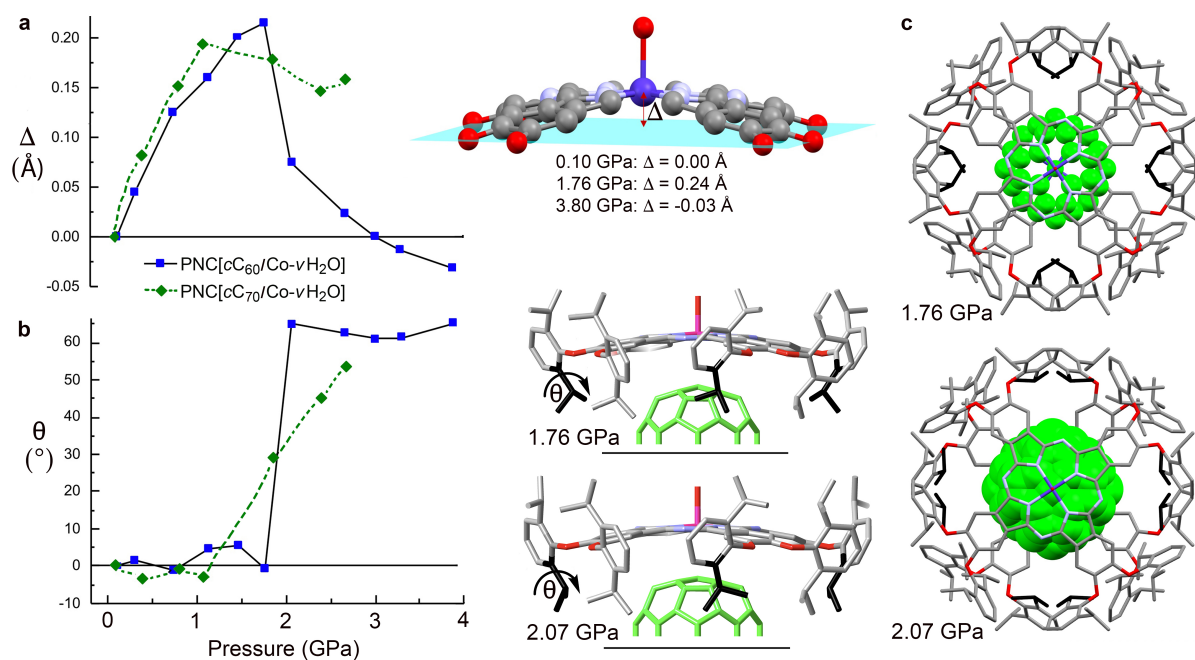
Fig. 3. Changes in molecular structure of the (dipPhO) 8 PcCo component on compression of PNC[ c C 60 /Co- \nu H 2 O] and PNC[ c C 70 /Co- \nu H 2 O]. (a) The change on increasing pressure of the distance, \Delta , between the Co atom and the mean position of the plane containing the eight O atoms on the periphery of the phthalocyanine. The substituents are removed for clarity. (b) The change in the torsion angle, \theta , of the iso -propyl groups, shaded black, which undergoes conformation rearrangement during the structural transformation of PNC[ c C 60 /Co- \nu H 2 O] between 1.76 and 2.07 GPa. (c) A view parallel to the parallel to the \bar{4} axis (i.e. looking down the axial Co-O bond) showing the increase between 1.76 and 2.07 GPa in the C 60 anisotropic displacement parameters (average U_{eq} value increase from 0.26 Å 2 to 0.94 Å 2 ).
