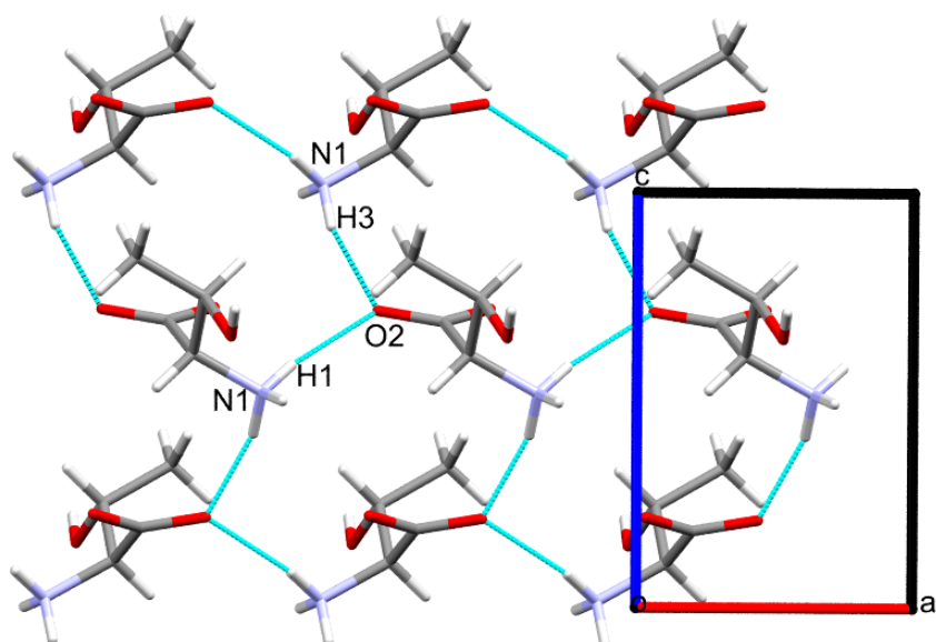
Figure 5 Hydrogen bonding in L-threonine at ambient pressure as viewed along b
