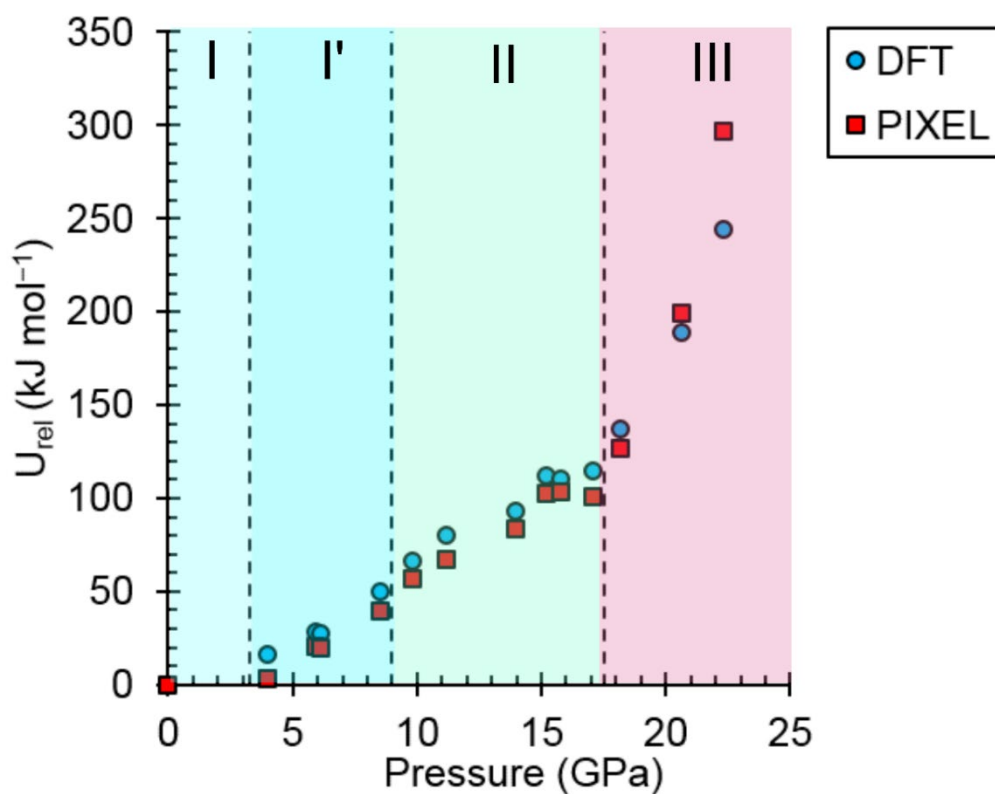
Figure 7 The variation of the lattice energy of threonine with pressure. The points are relative to ambient pressure ( U_{rel} ).
