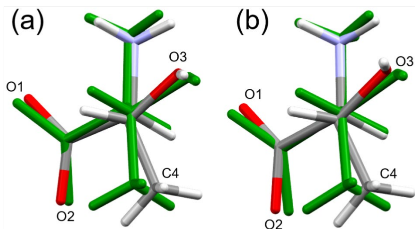
Figure 3 Structure overlay of the two symmetry-independent molecules of threonine at 22.3 GPa (coloured by element) [(a) molecule A and (b) molecule B] with the molecule at ambient pressure (coloured green). The view is down the C3-C2 bond. Overlay of the structures was determined using the structure overlay feature in MERCURY from atoms C1, C2 and C3 only.
