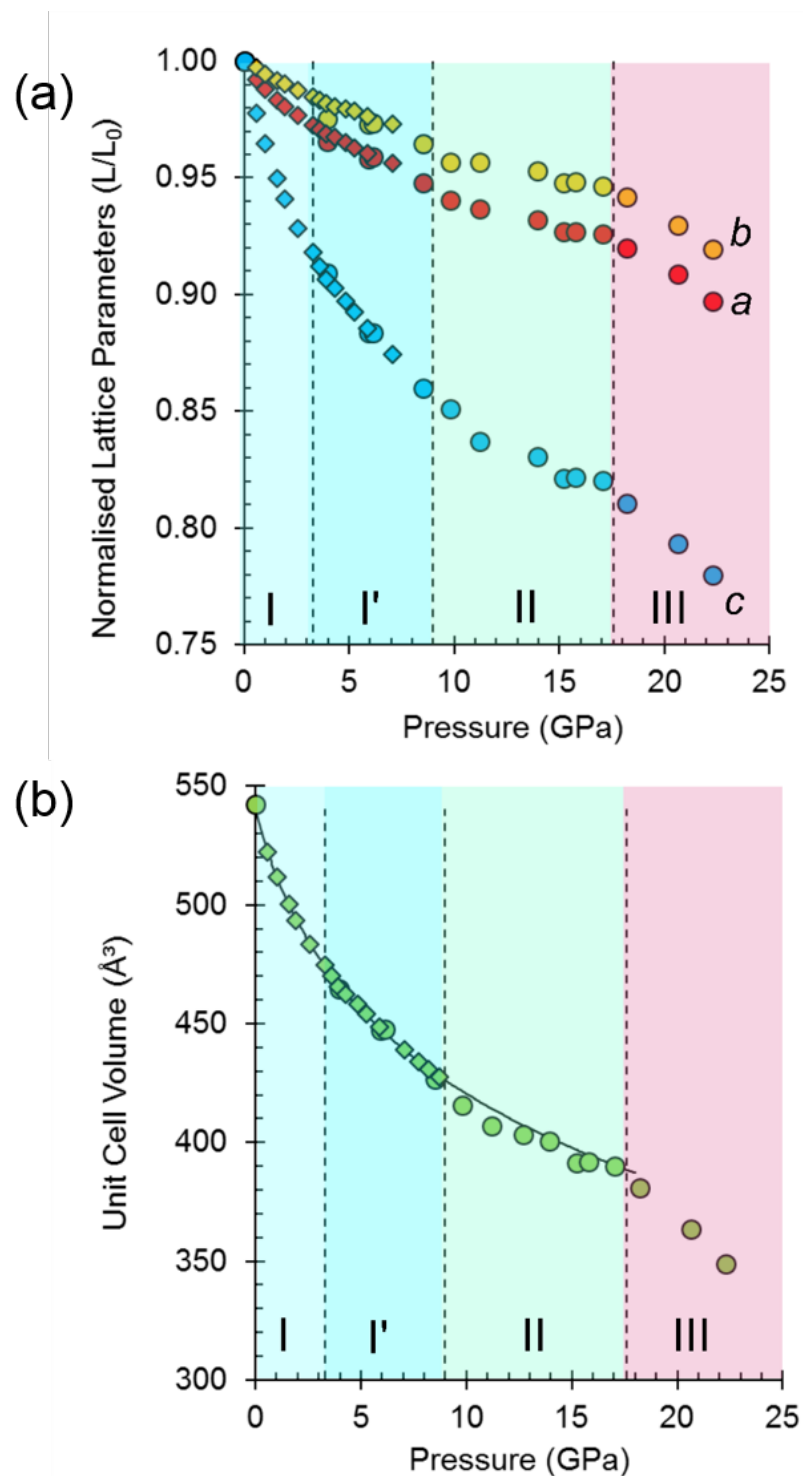
Figure 2 Variation of (a) the normalised lattice parameters and (b) unit cell volume of L-threonine as a function of pressure. Neutron data, collected using the d_8 isotopologue, are shown as diamonds. X-ray diffraction data, collected using isotopically normal threonine, are shown as circles. There is little evidence of any isotopic effect at the resolution of these experiments. The curve is the equation of state of phase I and I'.
