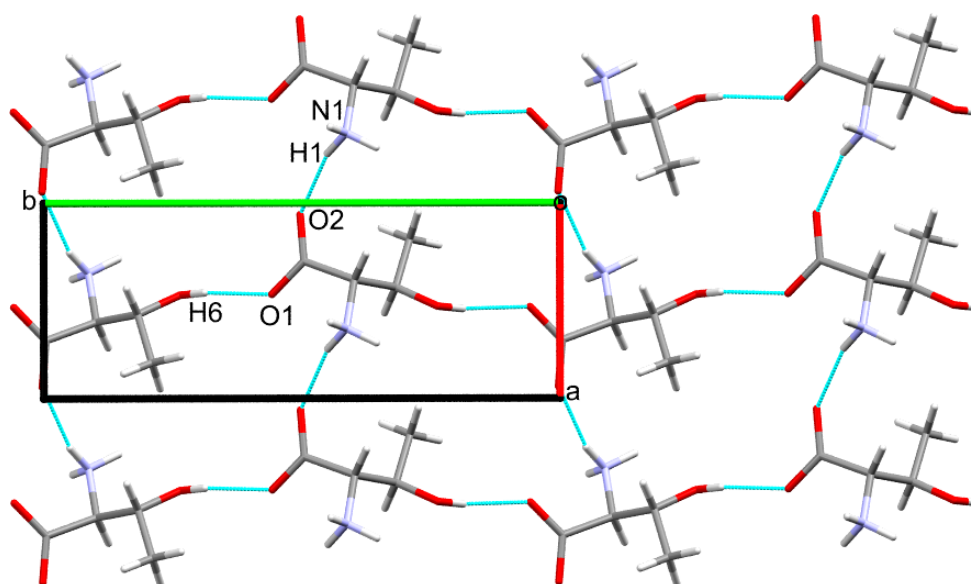
Figure 6 Hydrogen bonding in L-threonine at ambient pressure, as viewed along c
