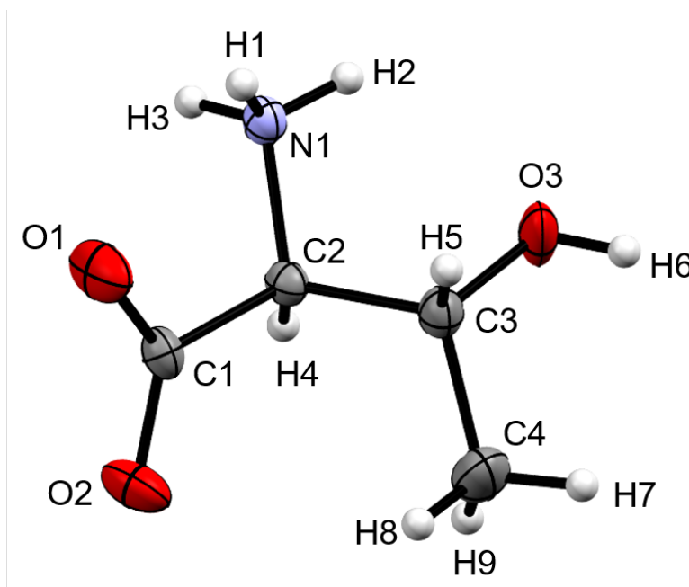
Figure 1 Molecular structure of L-threonine at ambient conditions showing the numbering scheme used. Ellipsoids are shown at the 50 % probability level.
