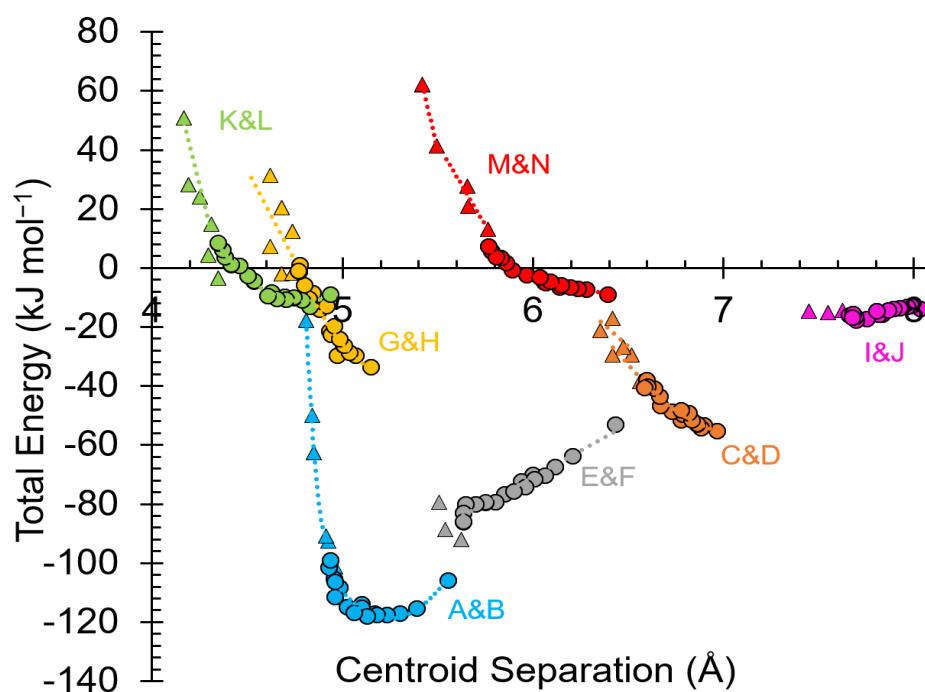
Figure 8 Molecular interaction energies of contacts A-N as a function of centroid separation. Circles represent phases I to II ( P2_12_12_1 ), and triangles represent phase III ( P2_1 ). The dotted lines have no functional significance and are meant to guide the eye.
