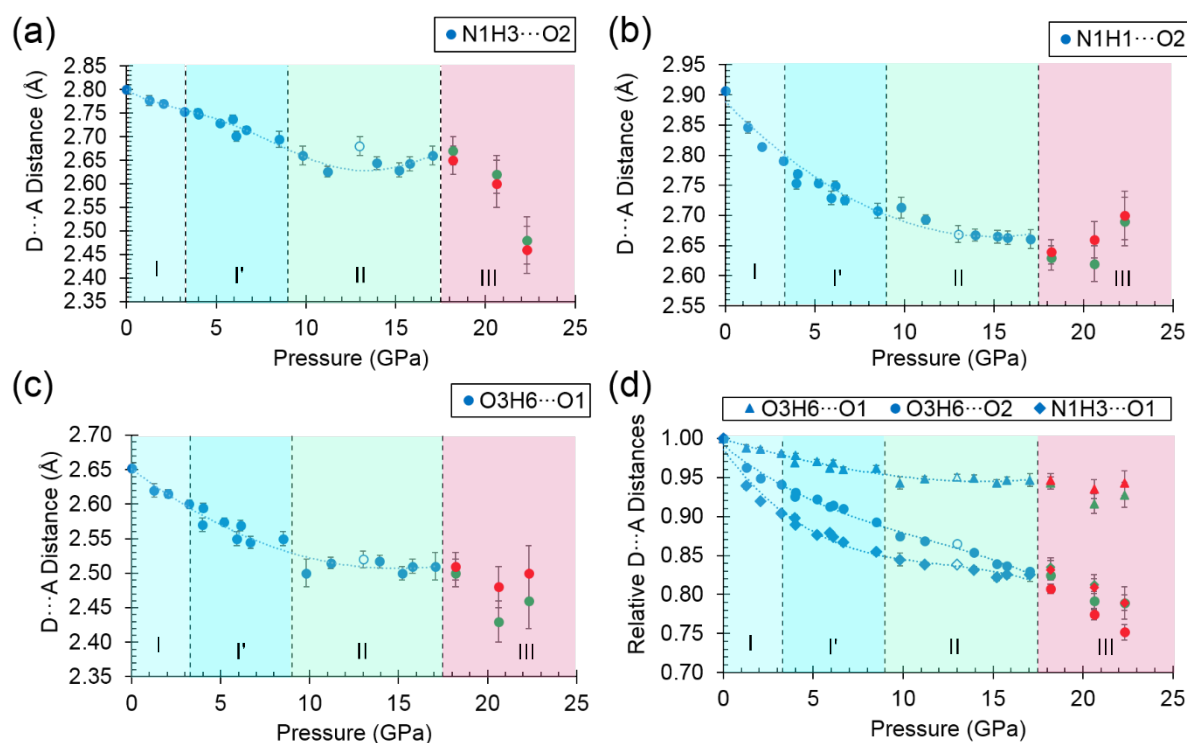
Figure 9 (a)–(d) Donor–acceptor distances of selected hydrogen bonds as a function of pressure, Decompression measurements at 13.0 GPa are represented by open markers. Molecules A and B in phase III are represented by green and red markers respectively. Trendlines are meant to guide the eye only.
