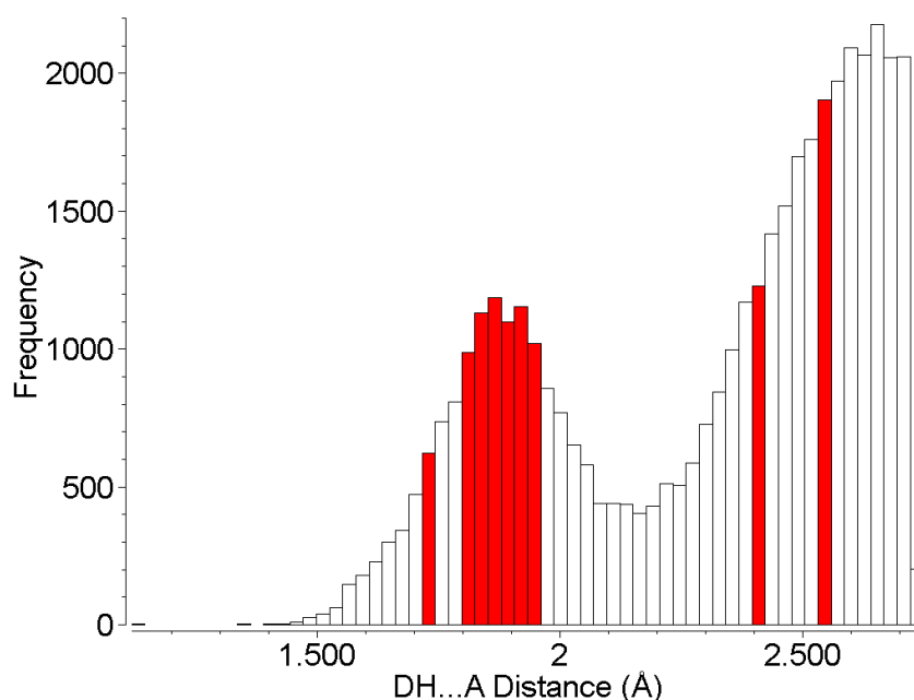
Figure 10. Hydrogen bond distances formed in the crystal structures of amino acids. Red bars show H-bond distances observed in L-threonine at 22.3 GPa.
