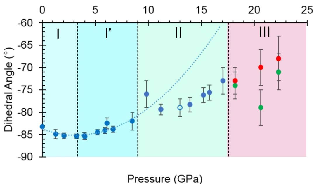
Figure 4 The O2-C1-C2-C3 torsion angle ( \tau ) as a function of pressure. The green and red circles in phase III represent molecules A and B, and the open circle represents the decompression measurement. A second order polynomial was fitted to phase I and I' data, the minimum of the parabolic function was determined to be -85.0^\circ at 3.3 GPa. Extrapolating the curve to 17.1 GPa serves to highlight the slower rate of change exhibited in phase II. Plots of other torsion angles against pressure are available in the ESI.
