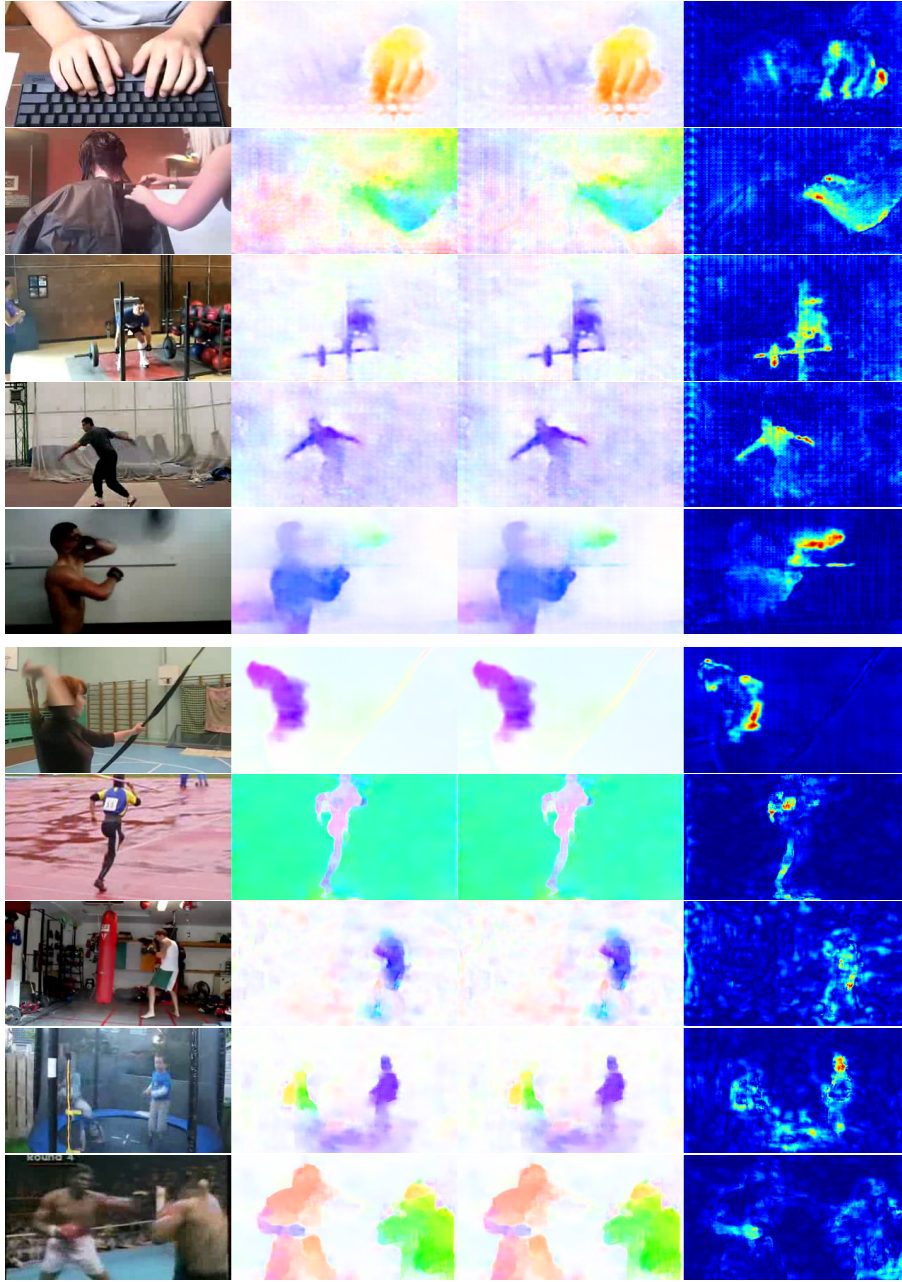
Fig. 5. Comparison of estimated flow fields from a network trained to minimize EPE and the same trained to minimize classification error. Top: Results from FlowNet. Bottom: Results from SpyNet. Each series of 4 images represent the first of the input images, the two flow fields, and the Euclidean distance between the two flow vectors at each pixel (red means higher distance, and blue means lower distance). Flow vectors noticeably change more around motion boundaries and where humans are located. In the case of FlowNet we observe the appearance of a checker-board pattern attributed to the upconvolution 9 , but we observe that it does not affect the improvement of performance for action recognition. SpyNet does not exhibit the artefact since it does not contain upconvolution.
