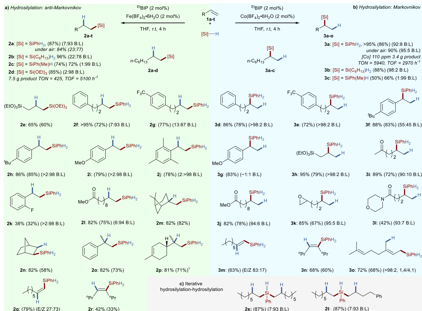
Scheme 2 Scope for iron- and cobalt-catalysed hydrosilylation reactions enabled by tetrafluoroborate activation. a) Reaction conditions: olefin, PhSiH 3 (1.1 eq.), E BIP (2 mol%) and Fe(BF 4 ) 2 •6H 2 O (2 mol%), THF, r.t., 4h. †M Me BIP (2 mol%) used. b) Reaction conditions: olefin, PhSiH 3 (1.1 eq.), E BIP (2 mol%) and Co(BF 4 ) 2 •6H 2 O (2 mol%), THF, r.t., 4h. c) Reaction conditions: alkene (1 equiv.), PhSiH 3 (1 equiv.), Fe(BF 4 ) 2 •6H 2 O (2 mol%), E BIP (2 mol%), THF, r.t., 30 min then a second alkene (1 equiv.) added, 3h. Yields determined by 1 H NMR spectroscopy of the crude reaction mixture using 1,3,5-trimethoxybenzene as an internal standard, isolated yields in parenthesis.
