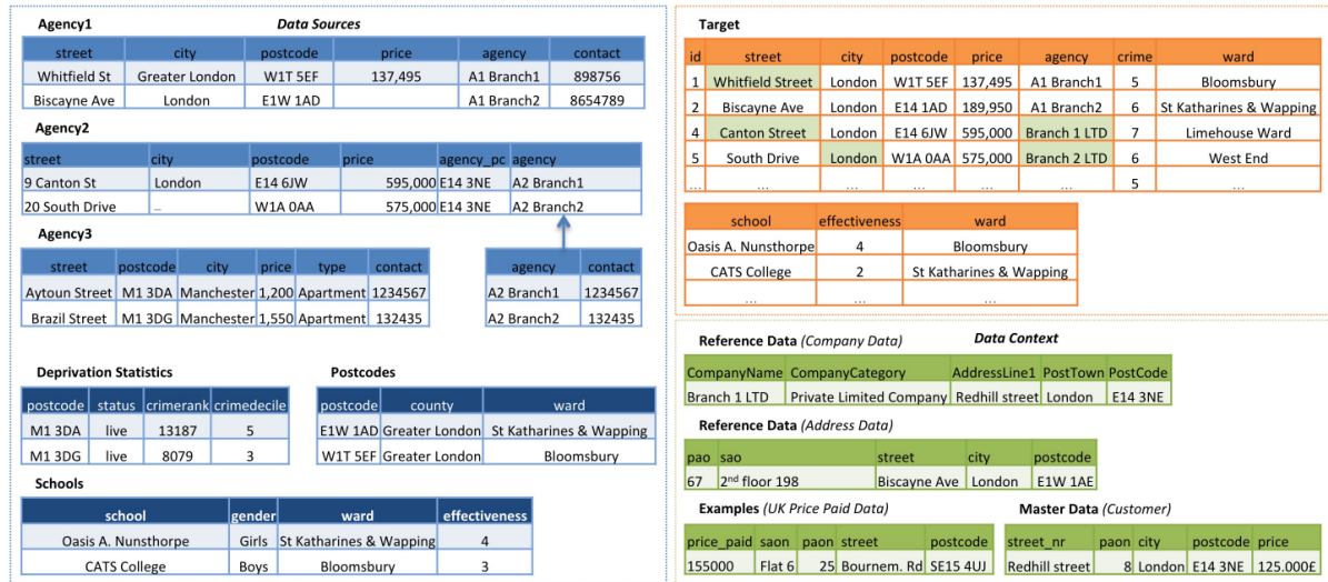
Fig. 1: Data wrangling scenario: collection of raw Web extracted real-estate sources and deprivation data (left-hand side) is wrangled into the target (right-hand side). Data context, i.e. reference data, master data and examples, informs the process of schema matching, value format transformation, data repair, and mapping generation, validation and selection.
