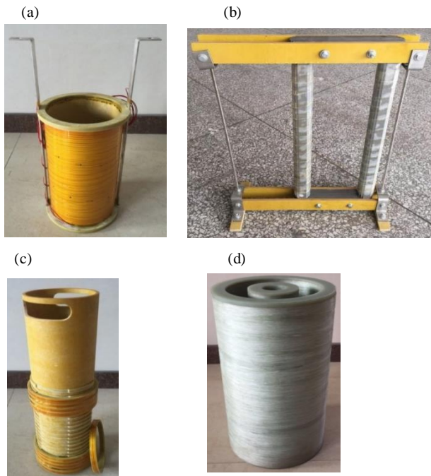
Fig. 3. Four parts of experiment prototype: (a) superconductor rings; (b) iron core; (c) current transmission/limiting coil; (d) cryogenic container
