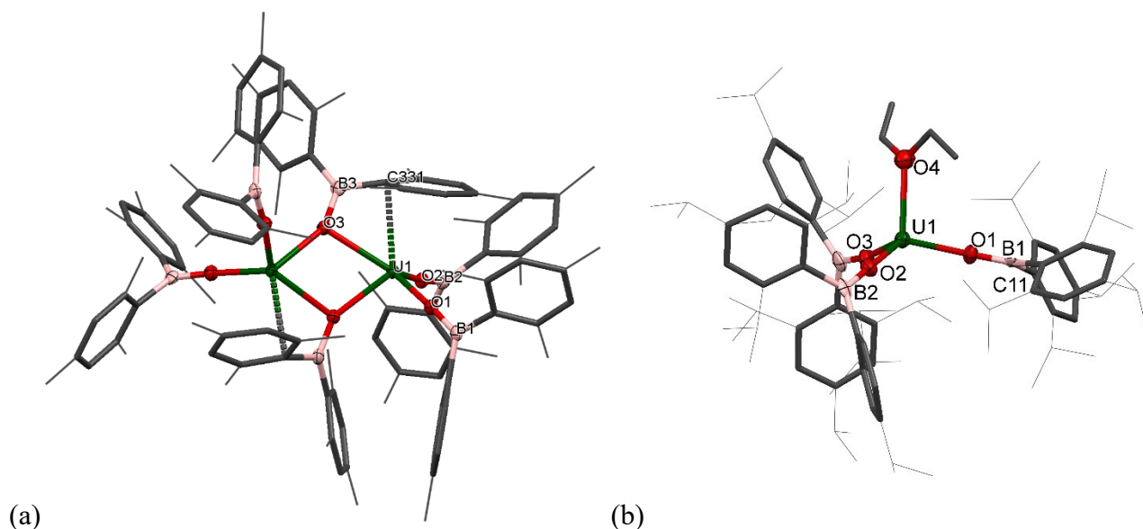
Figure 1 Displacement ellipsoid drawing of the molecular structure of (a) 1 m and (b) 1 t -Et 2 O . The methyl groups of the mesitylene are depicted as wireframe and the mesitylene groups as capped sticks for clarity. The hydrogen atoms are omitted. The thermal ellipsoids are displayed at 50% probability.
