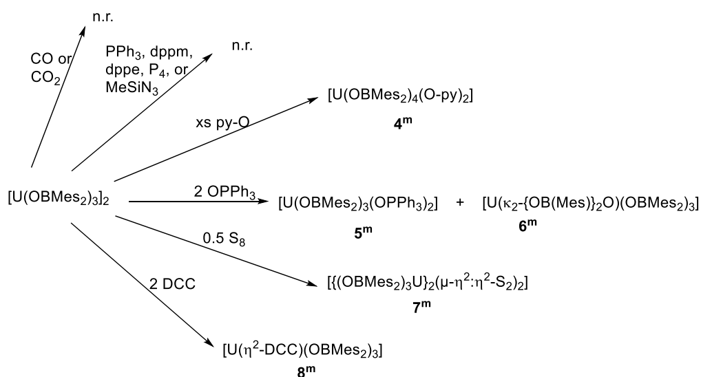
Scheme 2. Reactions of complex 1 m investigated.
