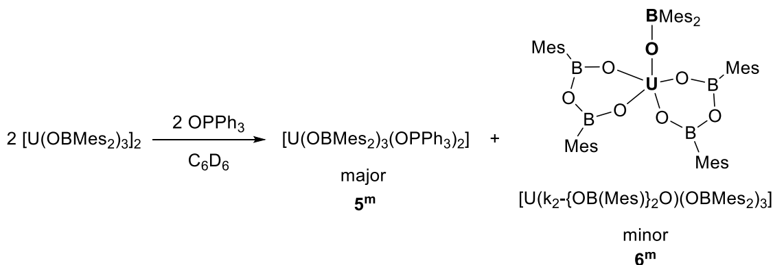
Scheme 3. Synthesis of compounds 5 m and 6 m .
