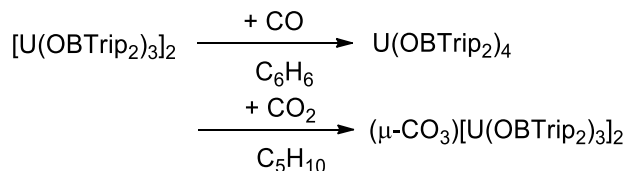
Scheme 4. Reactions of complex 1^t with CO and CO 2 .
