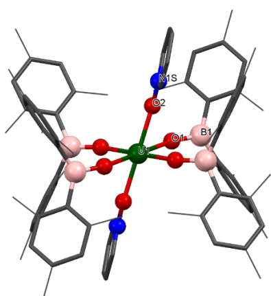
Figure 3. Solid-state structure of 4 m . Hydrogens atoms are omitted and mesitylene and pyridine oxide ligands are depicted as wireframe and capped sticks for clarity.
