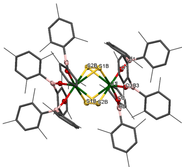
Figure 5. Solid-state structure of complex 7 m . Mesityl ligands are depicted as capped sticks and wireframe for clarity. Hydrogen atoms are omitted. The thermal ellipsoids are displayed at 50% probability.
