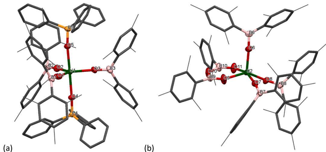
Figure 4. Solid-state structure of (a) \mathbf{5}^m and (b) \mathbf{6}^m . Mesitylene and phenyl ligands are depicted as capped sticks and wireframe for clarity. Hydrogen atoms are omitted. The thermal ellipsoids are displayed at 50% probability.
