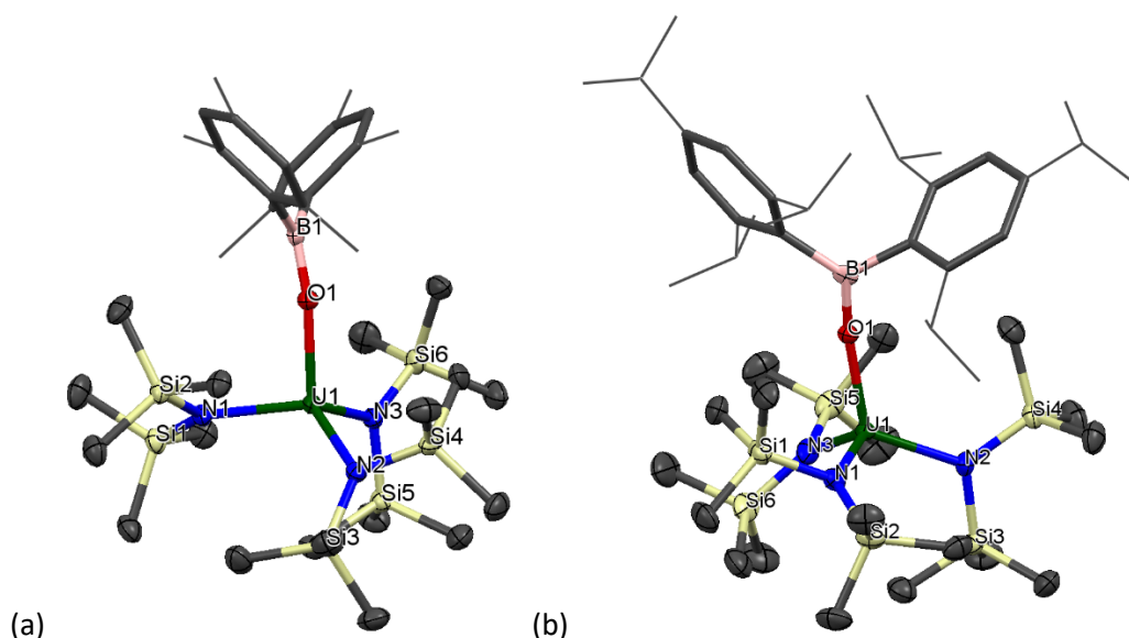
Figure 6. Solid-state structure of (a) 11 m and (b) 11 t . Mesityl and triisopropylphenyl ligands are depicted as capped sticks and wireframe for clarity. Hydrogen atoms are omitted. The thermal ellipsoids are displayed at 50% probability.
