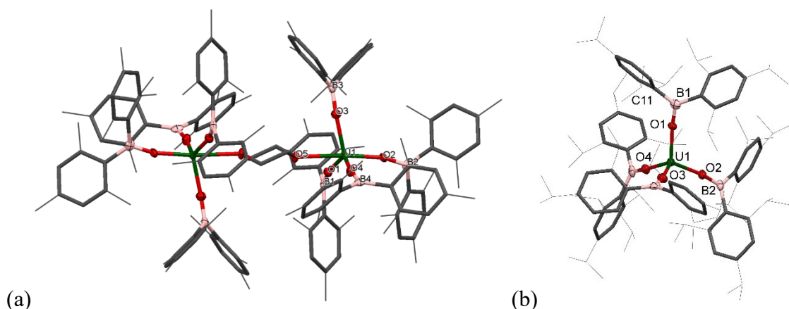
Figure 2 Displacement ellipsoid drawing of the molecular structure of (a) 2 m .diox and (b) 2 t ·2C 6 H 6 . Thermal ellipsoids are displayed at 50% probability. Lattice solvent and hydrogen atoms omitted, and aryl substituents are depicted as wireframe for clarity.
