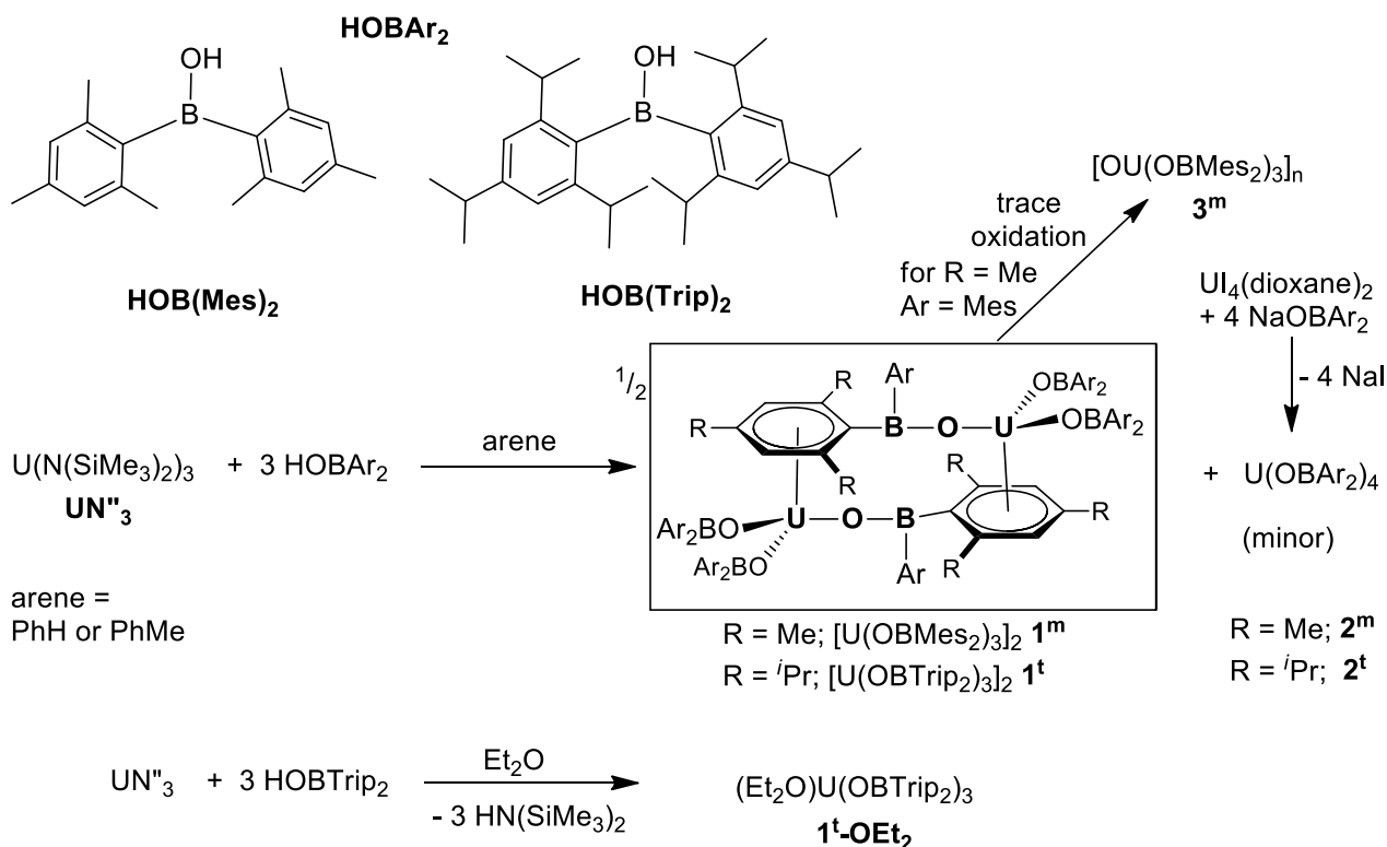
Scheme 1 Synthesis of complexes 1 showing common by-products and decomposition products
