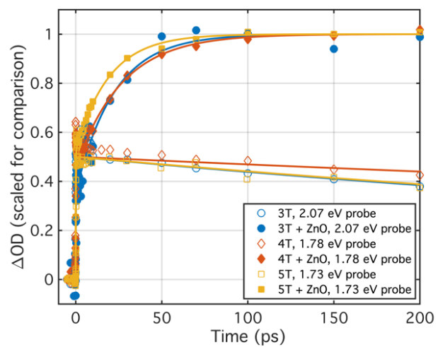
Figure 5. Scaled transient absorption intensities of 3T , 4T and 5T in CH 2 Cl 2 solution with and without ZnO NCs.
