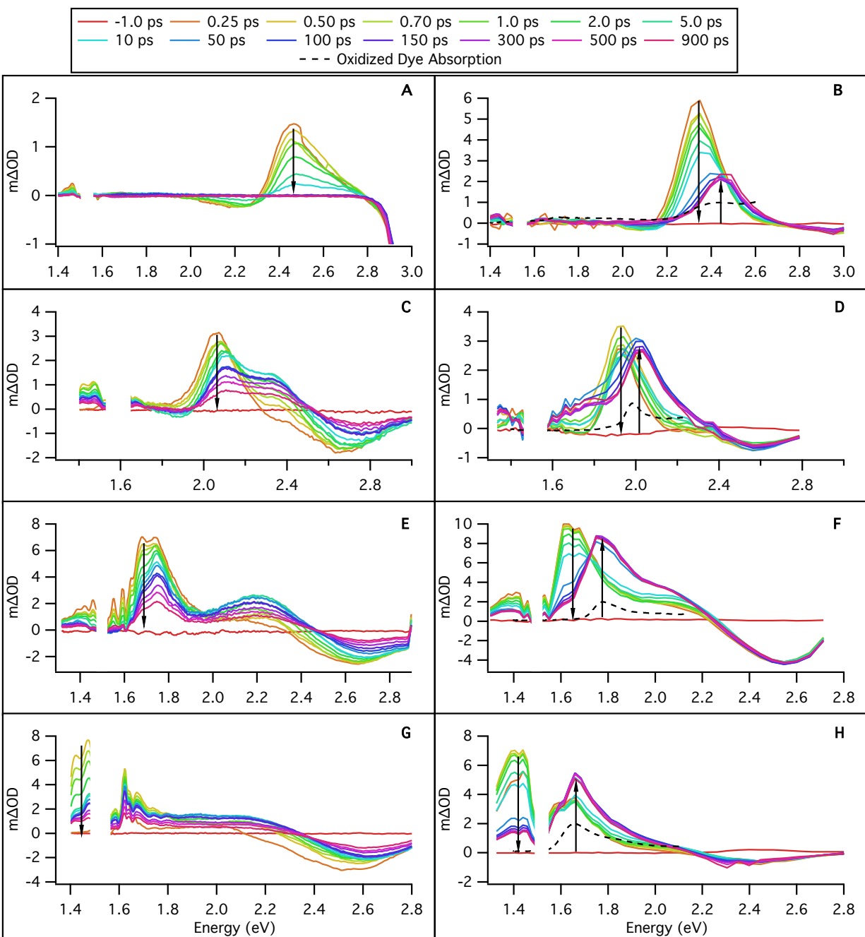
Figure 4. Ultrafast data for A) 2T alone in \text{CH}_2\text{Cl}_2 B) 2:1 2T to ZnO C) 3T alone in \text{CH}_2\text{Cl}_2 D) 2:1 3T to ZnO E) 4T alone in \text{CH}_2\text{Cl}_2 F) 2:1 4T to ZnO G) 5T alone in \text{CH}_2\text{Cl}_2 H) 2:1 5T to ZnO. Each color corresponds to the averaged \Delta\text{OD} in the visible range for a selection on time delays between the pump and probe in picoseconds. The blank space around 1.55 eV is due to residual light from the fundamental in the continuum probe. For the oxidized dye absorption, peaks are shown only for the oxidized dye and any ground state dye absorption has been omitted.
