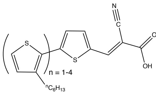
Figure 1. Molecular structures of 2T ( n = 1 ), 3T ( n = 2 ), 4T ( n = 3 ) and 5T ( n = 4 ).
