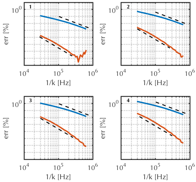
Figure 6: Convergence of the first four eigenfrequencies of the medium beam, for scheme (42) (blue) and (45) (red). Black dashed lines of slope 2 and 4 are also drawn, for reference.
