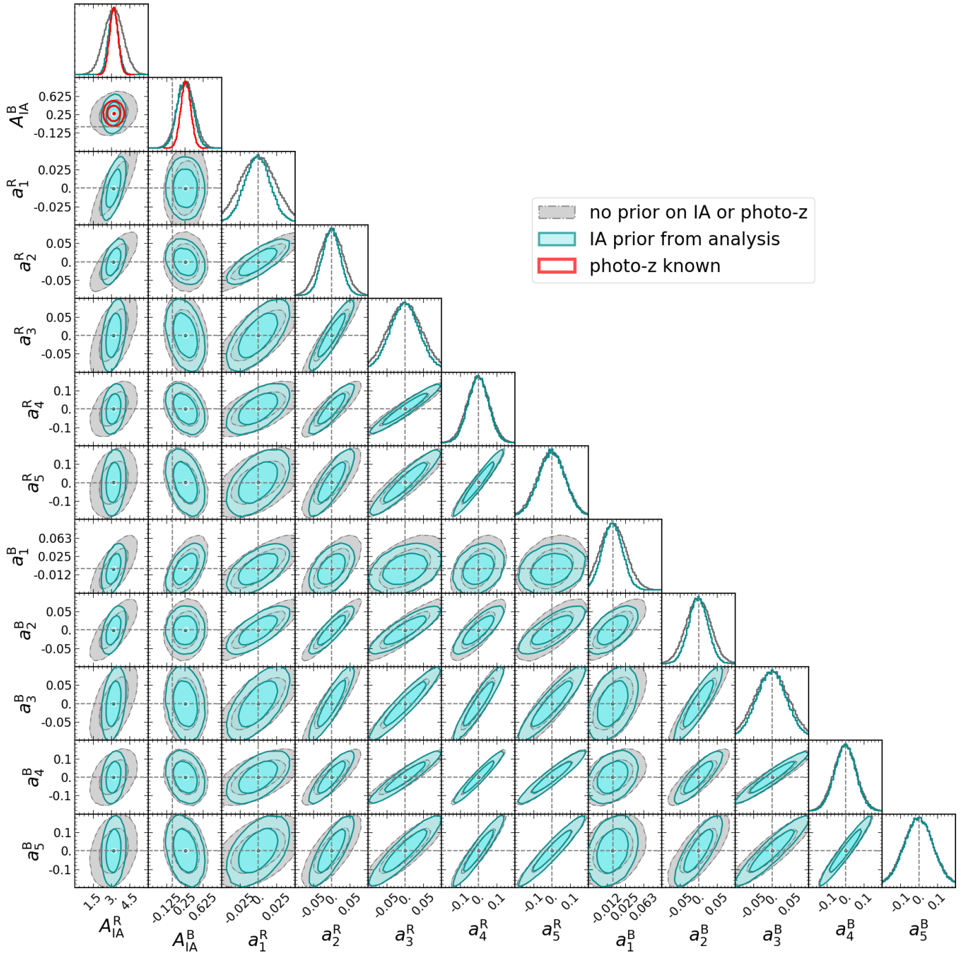
Fig. D.1. The same as Figure 8, for nuisance parameters only.
