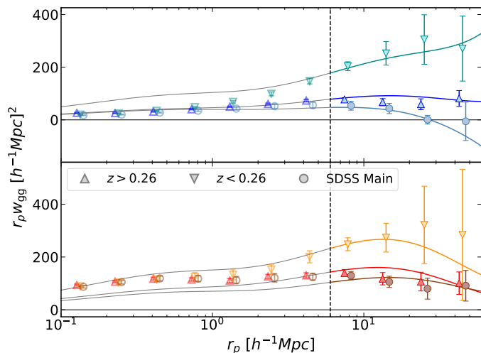
Fig. 2. Measured galaxy clustering for our blue ( top ) and red ( bottom ) galaxy samples. Solid curves illustrate the best-fit linear clustering per sample (Eq. 3.10). The vertical dashed line indicates r_p = 6 h^{-1}\text{Mpc} , below which scales are excluded from fitting (Section 3.3).
