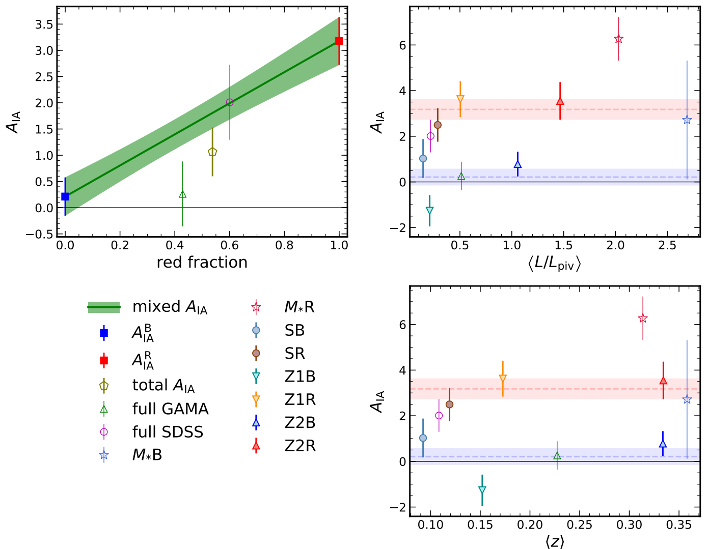
Fig. 6. Constraints on the NLA model alignment amplitude A_{\text{IA}} , from various subsamples of GAMA and SDSS (Table 1), plotted against sample properties. The constraints illustrated here are also given in Table B.1
