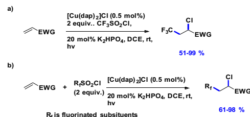
Fig. 18 Photoredox atom transfer radical addition reactions of fluoroalkylsulfonyl chlorides with electron-deficient alkenes 84
