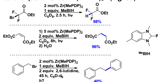
Fig. 39 Reactions tested using Zr^{(Me)PDP}_2 as photocatalyst.
