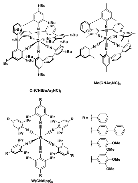
Fig. 11 Chromium, molybdenum, tungsten isocyanide complexes
