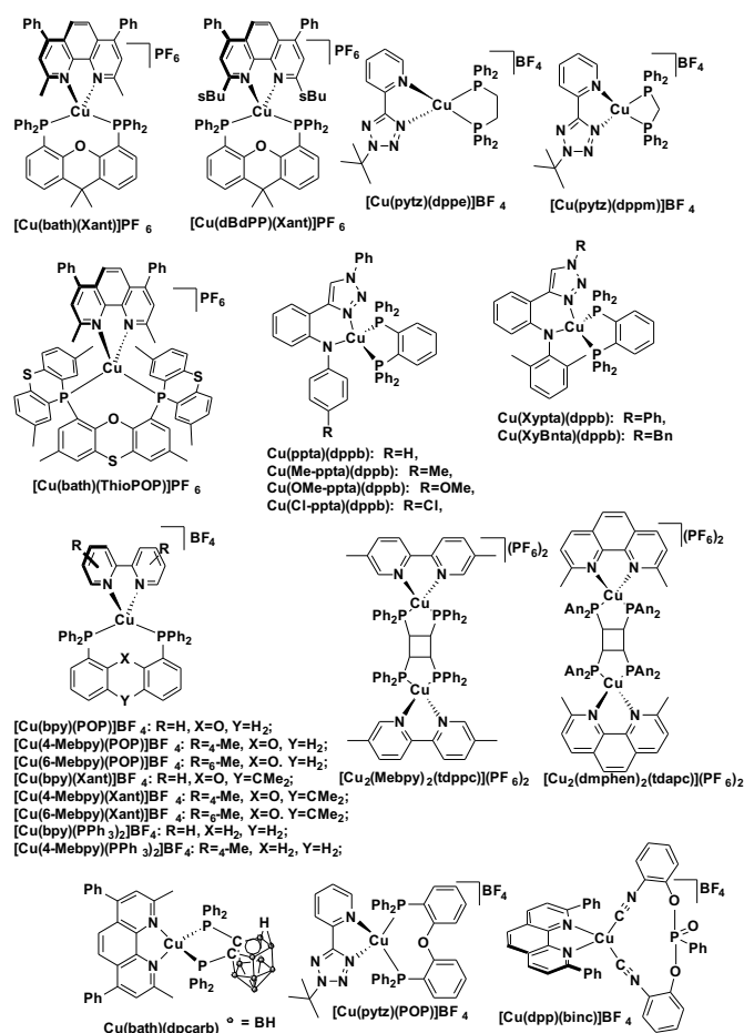
Fig. 6 [\text{Cu}(\text{N}^{\text{A}}\text{N})(\text{P}^{\text{A}}\text{P})]^+ and [\text{Cu}(\text{N}^{\text{A}}\text{N})(\text{P}^{\text{A}}\text{P})] type complexes.
