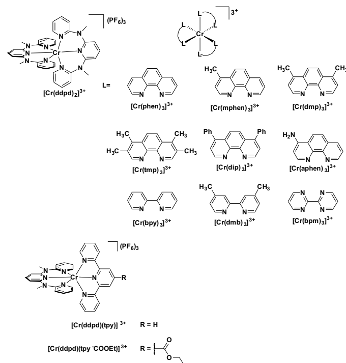
Fig. 34 Chromium (III) complexes.
