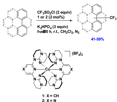
Fig. 46 Reaction conditions, catalyst structure and proposed mechanism for photocatalysis using a Co(III) complex.
