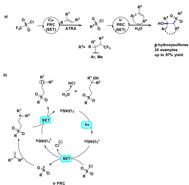
Fig. 15 Synthesis of \beta -hydroxysulfones from sulfonyl chlorides and alkenes 82 , Cu PC (SET) see Fig. 14b.
