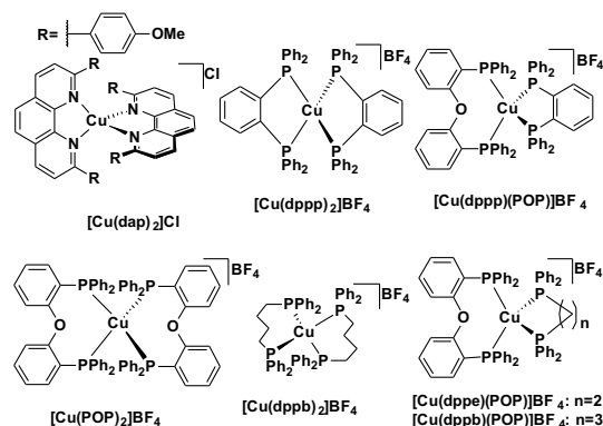
Fig. 7 [\text{Cu}(\text{N}^{\text{A}}\text{N})_2]^+ and [\text{Cu}(\text{P}^{\text{A}}\text{P})_2]^+ complexes.
