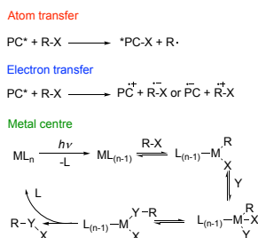
Fig. 2 Different possible mechanisms of photoredox catalysis.
