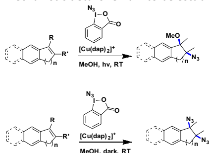
Fig. 25 Three-component azidation of styrene-type double bonds. 90
