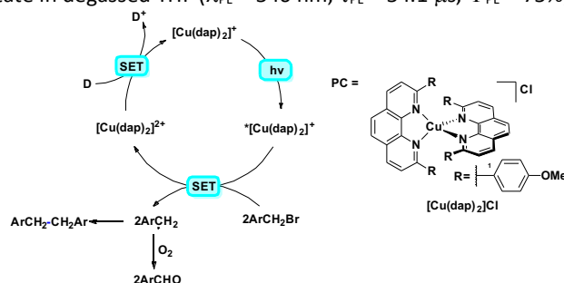
Fig. 12 Photoredox catalyzed reaction using a copper(I) complex reported by Sauvage et al. D represents an electron donor such as alkyl amines 46
