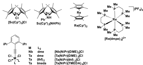
Fig. 29 Luminescent Rhenium, Scandium, Niobium, Tantalum complexes.
