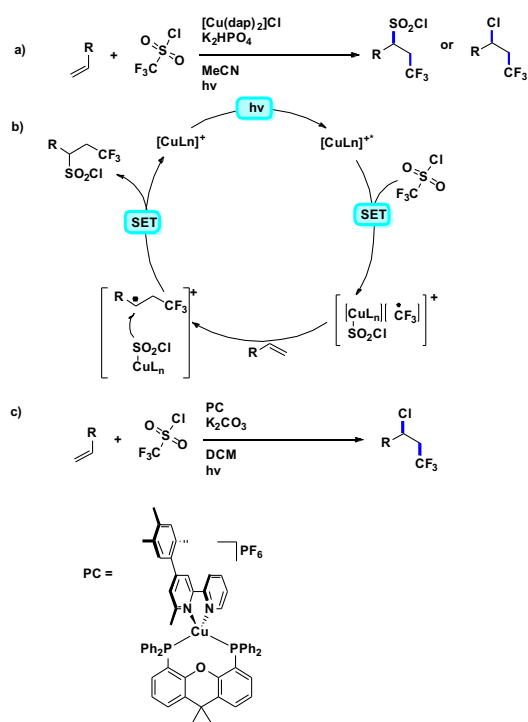
Fig. 14 Visible-light-induced [\text{Cu}(\text{dap})_2]\text{Cl} catalyzed trifluoromethylations of alkene.
