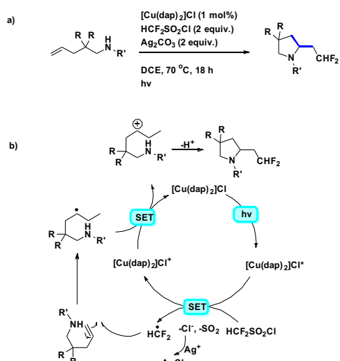
Fig. 19 Photoredox-catalyzed intramolecular aminodifluoromethylation of unactivated alkenes 85
