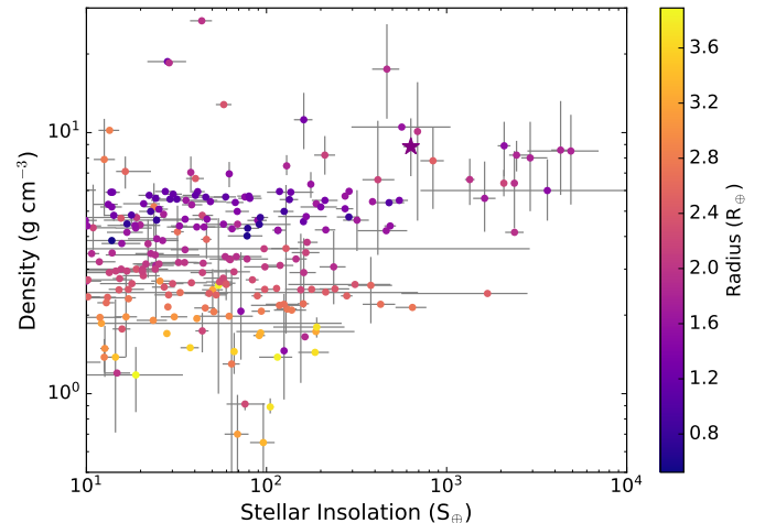
Figure 8. Density vs. stellar insolation for planets with radii smaller than 4 R_{\oplus} . Point color indicates the radius of the planet. K2-291 b (star) exhibits a density similar to other small, close-in planets.
