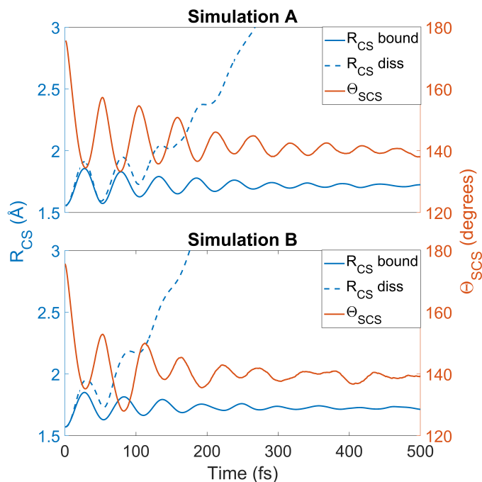
Fig. 8 Average R_{CS} for bound and dissociated molecules and average \Theta_{SCS} for bound molecules, calculated for simulation A (upper) and B (lower) as a function of time. The average bound geometry is calculated for all molecules up until they dissociate (i.e. CS fragments are excluded). The average \Theta_{SCS} is calculated from all trajectories as long as they remain intact (not dissociated). A trajectory is designated as dissociated when one R_{CS} exceeds the minimum distance from which dissociation is irreversible in each simulation.
