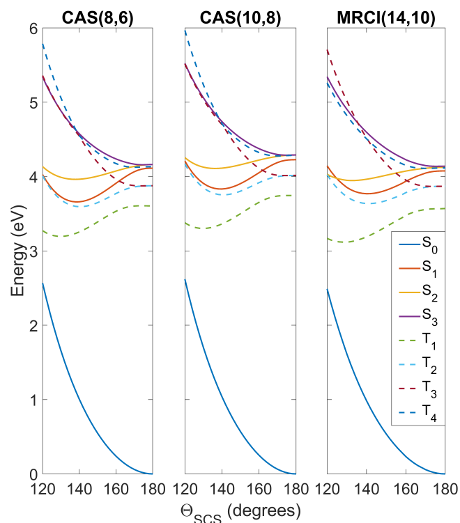
Fig. 3 Potential energy curves as a function of the \Theta_{SCS} bending coordinate, calculated at the SA8-CAS(8,6)/SVP (simulation A ), SA8-CAS(10,8)/SVP (simulation B ), and MRCI(14,10)/aug-cc-pvTZ (reference) levels of theory, shown in the left, center and right panels. Bond lengths are fixed at the CASSCF(16,12)/aug-cc-pvQZ optimised value of 1.569 Å. For compactness, only the range 120^\circ \leq \Theta_{SCS} \leq 180^\circ is shown as the curves are symmetric about the linear geometry at \Theta_{SCS} = 180^\circ . Here the states are labelled adiabatically. A full conversion table of adiabatic and diabatic state labels is given in Table 2.
