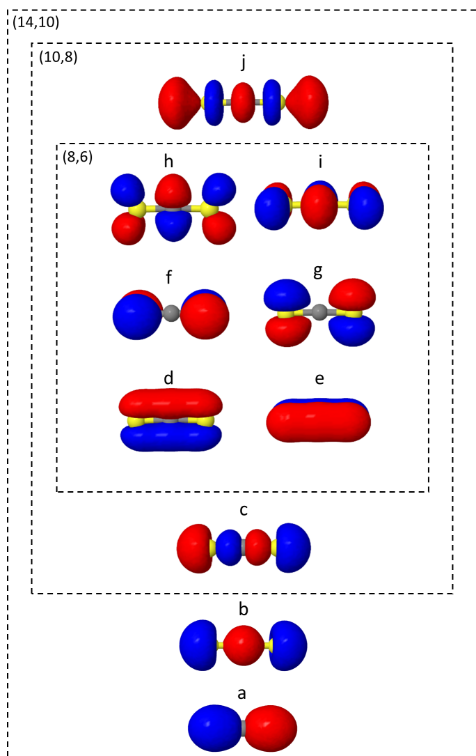
Fig. 2 Molecular orbitals (MOs) included in the active spaces (8,6), (10,8), and (14,10), corresponding to simulation A ( d-i , inner rectangle), simulation B ( c-j , center rectangle), and the reference calculations ( a-j , outer rectangle). The innermost (8,6) MOs ( d-i ) include the degenerate sulfur lone pair HOMOs, the \sigma bonding MOs and a \pi^* LUMO pair. The (10,8) active space includes a further two MOs ( c and j ) that correspond to an additional electron pair found in the next-highest occupied MO and a \sigma^* antibonding virtual MO. Finally, in (14,10) two occupied orbitals ( a and b ) are added.
