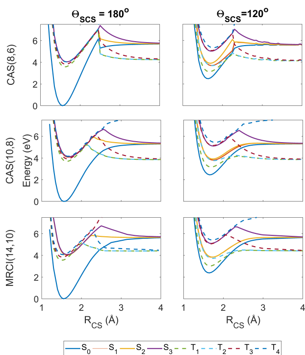
Fig. 4 Potential energy curves as a function of the R_{CS} stretch coordinate, with the second bond length fixed at R_{CS} = 1.569 \text{ \AA} and the angle \Theta_{SCS} fixed at linear 180^\circ (left column) and bent 120^\circ (right column), with calculations at the SA8-CAS(8,6)/SVP (simulation A ), SA8-CAS(10,8)/SVP (simulation B ), and MRCI(14,10)/aug-cc-pvTZ (reference) level shown in the top, middle and bottom rows. Here the states are labelled adiabatically. A full conversion table of adiabatic and diabatic state labels is given in Table 2.
