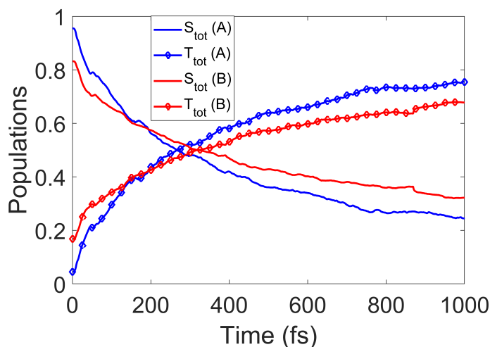
Fig. 5 Total singlet and triplet populations (quantum) as a function of time, defined as as the sum of the squares the MCH state coefficients, for simulations A and B .
