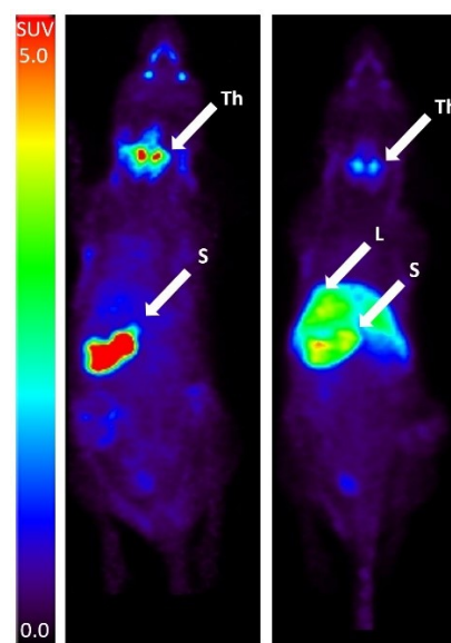
Figure 5. Comparison of [ 99m Tc]TcO 4 - uptake in naïve mice (left) vs. [ 99m Tc][TcO 4 C-2] 11+ (right). Free [ 99m Tc]TcO 4 - was injected into a naïve anaesthetised animal 40 minutes prior to a 20 minute SPECT acquisition. Caged [ 99m Tc]TcO 4 - was injected into a naïve anaesthetised animal 20 minutes prior to a 100 minute SPECT acquisition. Encapsulation results in reduced thyroid and stomach uptake, and increased liver uptake. Images are maximum intensity coronal projections. Additional examples are provided in the Supporting Information. S=Stomach, Th = Thyroid, L=Liver.
