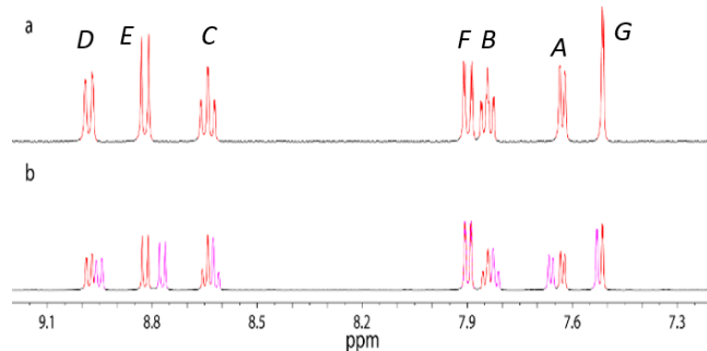
Figure 2. ^1\text{H} NMR spectra (500 MHz, \text{D}_2\text{O} , 298 K) showing the encapsulation of \text{ReO}_4^- by \text{C-1}^{12+} . (a) \text{C-1} \cdot 12\text{NO}_3 only; (b) \text{C-1} \cdot 12\text{NO}_3 + \text{NH}_4\text{ReO}_4 (free cage signals in red, occupied in pink). The assignments correspond to lettering shown in Figure 1a.
