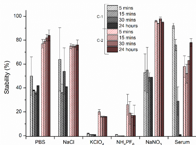
Figure 4. Stability of encapsulated complexes to different anions and conditions. 100 \mu\text{M} solution of salt was added to each cage made at their respective EC 95 (100 \mu\text{M} for C-1 and 1.9 \mu\text{M} for C-2). For details see Supporting Information.
