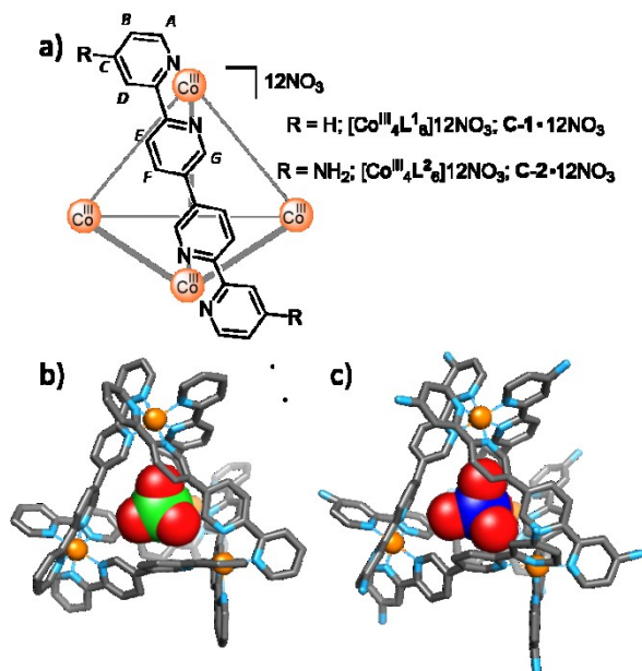
Figure 1. (a) Chemical structure of anion-binding \text{Co}^{\text{III}}_4\text{L}_6 cages (only one ligand shown for clarity); X-ray crystal structures of (b) [\text{ClO}_4\text{-C-1}]^{11+} ; (c) [\text{ReO}_4\text{-C-2}]^{11+} . Non-encapsulated anions and solvent molecules removed for clarity. Color Code: Co, orange; C, grey; N, light blue; O, red; Cl, green; Re, dark blue.
