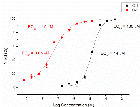
Figure 3. Radiochemical yield for [\text{C-1}]^{11+} encapsulation as a function of cage concentration ( \text{C-1} , black squares; \text{C-2} , red circles). For details see Supporting Information.
