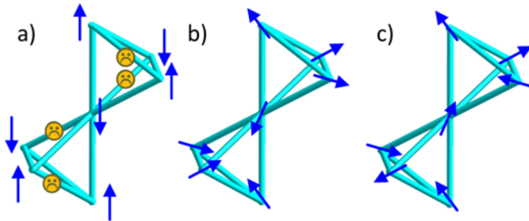
Figure 1. Frustrated magnetic order on a uniform pyrochlore lattice. Spins lie at the apices of a lattice of corner-sharing tetrahedra, and all nearest-neighbour couplings are of equal magnitude, as represented by the blue lines. (a) A ground state configuration for collinear spin order when nearest-neighbour couplings are antiferromagnetic. This ground state is highly degenerate but lattice distortion may stabilise one configuration. Four antiferromagnetic couplings are satisfied in each tetrahedron, and two are frustrated as indicated by ‘sad face’ symbols – this construct is useful for the more complex frustrated configurations shown in Fig. 4. (b) Non-collinear spin order for situation (a) can give rise to the ‘all-in all-out’ configuration where all magnetic moments point towards or away from the centre of each B-site tetrahedron, preserving cubic symmetry and with each antiferromagnetic coupling partly frustrated. (c) Strong dipolar interactions can lead to a related ‘2-in 2-out’ spin ice order with two spins pointing in and two pointing out of each tetrahedron when spin-spin couplings are weakly ferromagnetic. This is also shown as one of the magnetic phases for \gamma -Fe 2 SiO 4 in Fig. 5e.
