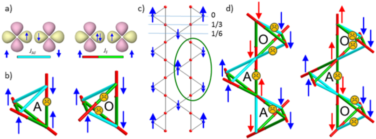
Figure 4 Frustration wave model for orbital and spin correlations. (a) Nearest-neighbour Fe 2+ -Fe 2+ t_{2g} orbital and magnetic interactions. The t_{2g}^1-t_{2g}^1 interaction (left) leads to antiferromagnetic coupling J_{AF} between cation spins shown in the lower corners and is represented by the light blue bar below and in (b) and (d). The t_{2g}^2-t_{2g}^1 interaction (right) shows t_{2g}^2 orbital order and associated ferromagnetic coupling J_F , respectively represented by red and green bars below and in (b) and (d). (b) The two configurations for orbital order and magnetic interactions within tetrahedra of four Fe 2+ cations. Four edges have orbital order and ferromagnetic couplings and two are antiferromagnetic. Tetrahedra with antiferromagnetic couplings on Adjacent (A, left hand image) edges have a 3 up/1 down spin ground state for J_{AF} \approx -J_F , where the two spins adjacent to the frustrated interaction are partially frustrated but the other are unfrustrated. The alternative configuration has antiferromagnetic couplings on Opposite (O, right hand image) edges and is uniformly frustrated with ferromagnetic and antiferromagnetic ground states of comparable energy for J_{AF} \approx -J_F ; the latter is shown here. (c) (\frac{2}{3} -\frac{2}{3} 0) approximant model for the Fe1 spin order in Fe 2 GeO 4 shown in Fig. 3c, projected on the [110] plane of the cubic spinel structure. Fe1 moments form ferromagnetic chains perpendicular to the image plane; one third have fully ordered up spins (Fe1:+S) and two thirds are partially-fluctuating down spins (Fe1:-S/2). Perpendicular ordered spins at Fe2 sites (red) are not shown. Values of the frustration index F in the different spin layers are shown. (d) Two fluctuating configurations for orbital and spin orders within the representative unit circled in (c). Static Fe1 spin components (blue) are coupled through dynamic components of the Fe2 spins (red). The central tetrahedron is always A-type and the two blue (Fe1:+S) spins have no frustrated interactions to nearest-neighbours and are fully ordered. The top and bottom tetrahedra fluctuate between A and O configurations and have (Fe1:-S/2) spins with some frustrated interactions. Fe2 spin components fluctuate between up and down in these and other configurations and have no static ordered component parallel to Fe1 spins.
