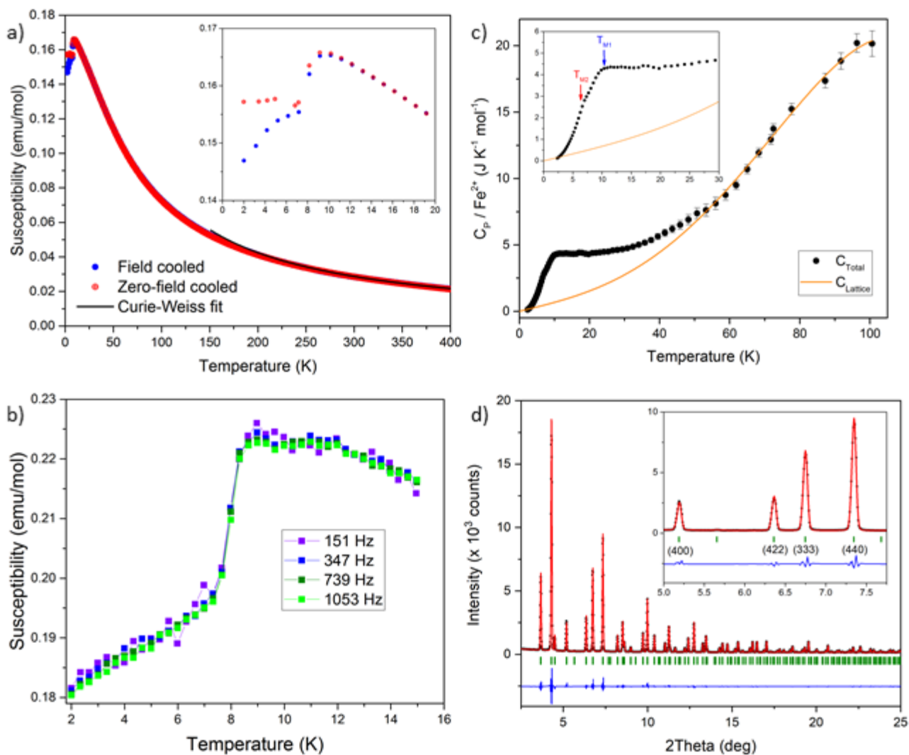
Figure 2. Magnetic and structural characterisation of \text{Fe}_2\text{GeO}_4 . (a) Magnetic susceptibility in an applied field of 0.5 T, with inset showing the low temperature region where magnetic transitions occur at T_{m1} \approx 9 K and T_{m2} \approx 7 K. The Curie-Weiss fit to points between 150 K and 400 K gives an effective paramagnetic moment of 4.25 \mu_B , consistent with high-spin 3d^6 \text{Fe}^{2+} spins, and a Weiss temperature of \theta = -19.6 K (b) Real part of the AC susceptibility in an oscillating magnetic field with amplitude 9 Oe and frequencies as shown. No frequency-dependence of the features that would evidence spin-glass behaviour is observed. (c) Heat capacity variation with the lattice contribution fitted by the polynomial C_p = \gamma T + \beta T^3 + \delta T^5 . The inset shows the low temperature region with discontinuities at T_{m1} and T_{m2} marked. The magnetic contribution is evident up to 55 K but the integrated entropy in the 2-55 K range of 5.77 \text{ J mol}^{-1}\text{K}^{-1} is only 43% of the theoretical R \ln(2S+1) = 13.38 \text{ J mol}^{-1} for S = 2 . Error bars are standard deviations. (d) Fit of the cubic spinel model to the synchrotron x-ray diffraction profile ( \lambda = 0.1917 \text{ \AA} ) at 5 K, with the region containing (400) and (440) reflections that are sensitive to a tetragonal lattice distortion shown in the inset. No peak splittings or broadenings that would evidence a lattice distortion are observed.
