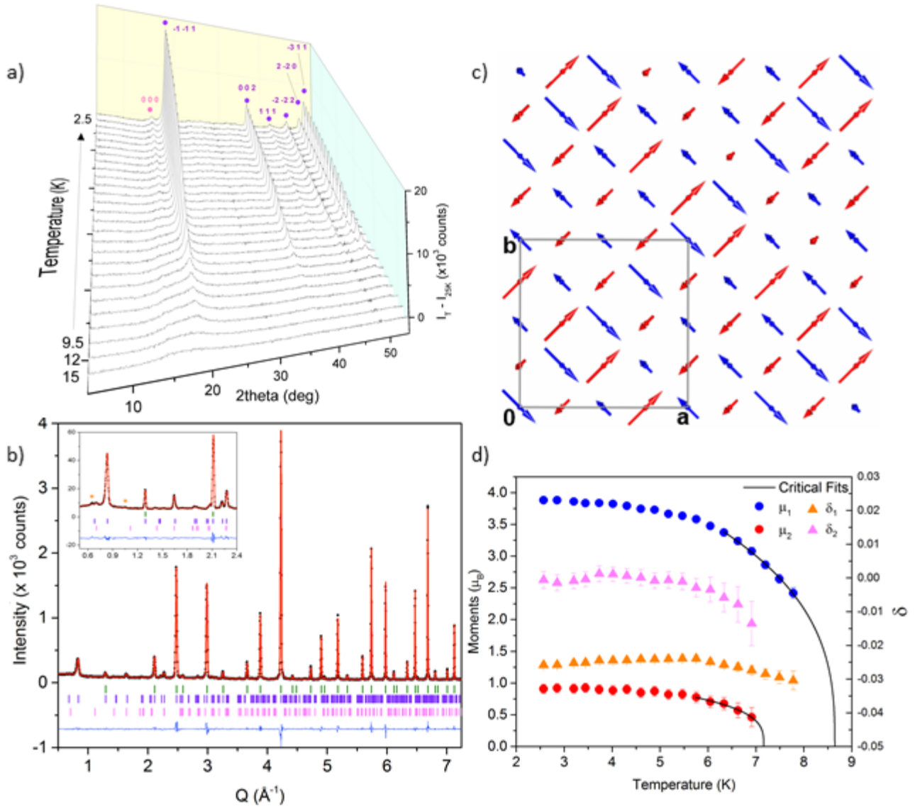
Figure 3 Low temperature neutron diffraction results for Fe 2 GeO 4 . (a) Magnetic scattering profiles obtained by subtracting the 25 K D20 data from profiles between 2.5 and 9.5 K, recorded in \sim 0.3 K steps, and at 12 and 15 K. hkl labels correspond to magnetic satellite reflections at (hkl) + \mathbf{k}_i for \mathbf{k}_i = (\frac{2}{3} + \delta_i \frac{2}{3} + \delta_i \mathbf{0}) . The five magnetic peaks with black labels that appear below T_{m1} = 8.9 K have propagation vector \mathbf{k}_1 , while the weak 000 peak indicated in pink appears below T_{m2} = 6.6 K with vector \mathbf{k}_2 . (b) Fit of the crystal and magnetic structures at 2 K, to high resolution D2B data at 2 K ( \lambda = 1.54 Å). The inset shows the fit in the low-angle region of D20 data ( \lambda = 2.41 Å). Two weak impurity peaks are labelled with asterisks. Magnetic reflection markers are in violet ( \mathbf{k}_1 ) and pink ( \mathbf{k}_2 ), and the structural reflections are in green. (c) The \mathbf{k}_1 order below T_{m1} with sinusoidal modulation of the Fe1 (blue) and Fe2 (red) moment amplitudes in the [1T0] and [110] directions respectively. Moments vary between 0 (fully frustrated) and 4 \mu_B (fully ordered) values. The additional \mathbf{k}_2 order below T_{m2} adds a small modulated tilting of the moments shown separately in Supplementary Fig. 6. (d) Temperature variations of the magnetic moments \mu and propagation vector contributions \delta for Fe1 and Fe2 with canting in the ab -plane. Fits of the critical law \mu = \mu_0(1 - T/T_m)^\beta to the moment variations are shown where \beta_1 = 0.35(6) and T_{m1} = 8.6(2) K and \beta_2 = 0.3(1) and T_{m2} = 7.2(2) K for the two transitions. Error bars are standard deviations.
