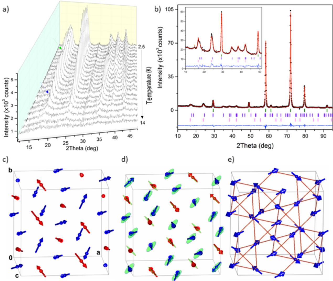
Figure 5 Low temperature neutron diffraction results for \gamma -Fe 2 SiO 4 . (a) Magnetic scattering profiles obtained by subtracting 25 K D20 data from profiles between 2.5 and 14 K, recorded in \sim 0.6 K steps. Blue and green arrows respectively show changes in diffraction intensity at the T_{m1} = 13 K and T_{m2} = 8 K transitions. (b) Fit of the crystal and magnetic structures at 2 K, to D20 data at 2K with 90^\circ takeoff angle. The inset shows the fit to prominent magnetic peaks in the low-angle region for data with 42^\circ takeoff angle to give high resolution. Magnetic reflection markers are in violet ( \mathbf{k}_1 ) and pink ( \mathbf{k}_2 ), and structural reflections are in green. A weak impurity peak is labelled with an asterisk. (c) Canted model for the \mathbf{k}_1 = (\frac{3}{4} + \delta, \frac{3}{4} + \delta, 0) order observed below T_{m1} , showing Fe1 (blue) and Fe2 (red) moments. (d) Alternative elliptical helix model for the \mathbf{k}_1 order, showing the planes of rotation for the moments. (e) The additional \mathbf{k}_2 = (1, 0, 0) ordered spin ice phase observed below T_{m2} , showing the tetrahedra of 2-in-2-out moments.
