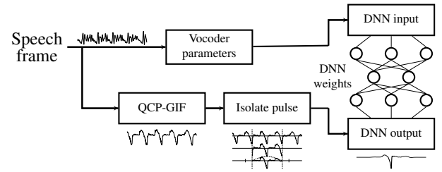
Fig. 3. DNN-based excitation generation framework.
