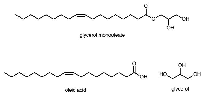
Fig. 1 The molecular structures of glycerol monooleate (GMO), oleic acid (OIH), and glycerol (Gly).
