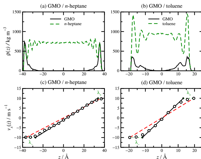
Fig. 5 Local density profiles and velocity profiles for GMO in n -heptane [(a) and (c)] and toluene [(b) and (d)]: (a) \rho(z) for GMO in n -heptane; (b) \rho(z) for GMO in toluene; (c) v_x(z) for GMO in n -heptane; (d) v_x(z) for GMO in toluene. z is the distance from the middle of the fluid layer. In (c) and (d), the MD simulation results are shown as unfilled circles, fits to eqn (3) as solid black lines, v_s z / H_z as red dashed lines, and \lambda_{\pm} as green dotted lines.
