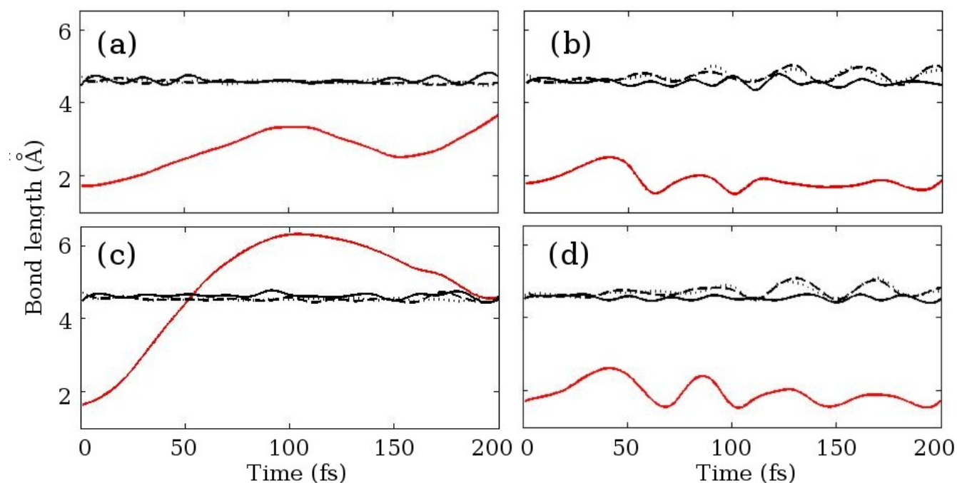
Fig. 5 Distances between the carbon atoms as a function of time for each of the trajectories (a,b,c,d) shown in the corresponding panels a-d. The distance between carbon atoms C_1 and C_6 , corresponding to the bond that is broken in the ring-opening reaction, is shown in red. Note that trajectories (a,c) are ring-opening and (b,d) are ring-closed. Three further nearest-neighbour C_i-C_{i\pm 1} distances are shown in black, but have been shifted by +3 Å to avoid congestion in the plots. The panels are labeled as follows: a) Trajectory a (direct to open; weight 0.2), b) Trajectory b (closed; weight 0.19), c) Trajectory c (rapid open; weight 0.18), and d) Trajectory d (closed; weight 0.14).
