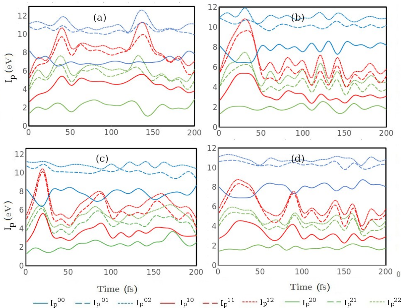
Fig. 8 Ionisation potentials I_p^{ij} = E_j - E_i as a function of time for each of the trajectories (a,b,c,d) shown in the corresponding panels a-d (labels as in Fig. 5). E_i is the potential energy of CHD in states i = 0, 1, 2 ( S_0 , S_1 and S_2 ) and E_j that of \text{CHD}^+ in states j = 0, 1, 2 ( D_0 , D_1 and D_2 ), resulting in nine channels overall. The channels that originate in S_0 , S_1 and S_2 , are shown in blue, red and green, respectively, and channels that correspond to excited states of \text{CHD}^+ ( j > 0 ) are shown as dashed lines.
