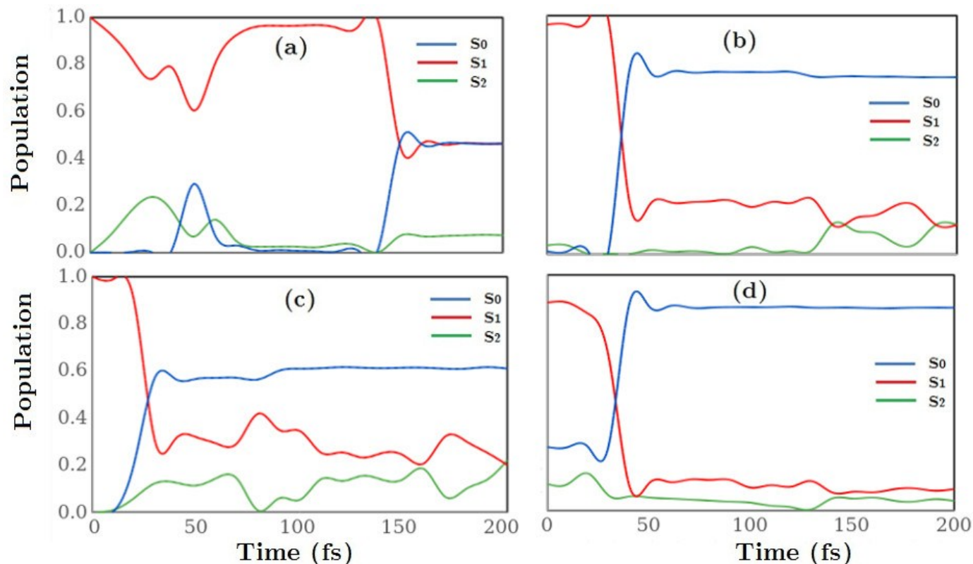
Fig. 6 Populations |a_k^i(t)|^2 in the electronic states i=S_0, S_1 , and S_2 as a function of time for the four trajectories (a,b,c,d) shown in panels a-d (labels correspond to Fig. 5).
