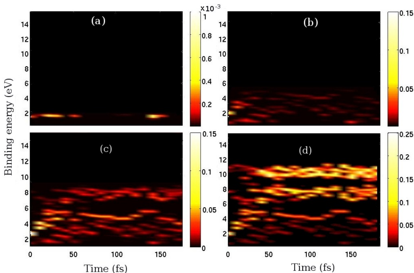
Fig. 10 Total photoelectron spectra (for all four trajectories combined) at probe energy: a) 2 eV, b) 6 eV, c) 9.2 eV, and d) 15 eV. The probe pulse envelope has Gaussian shape with bandwidth \approx 0.3 eV.
