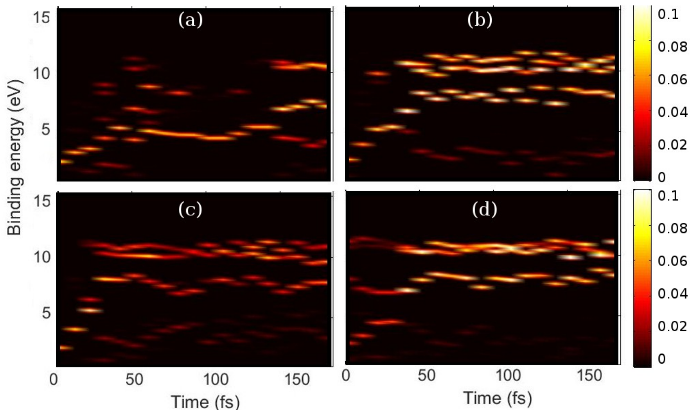
Fig. 11 Photoelectron spectra for each of the trajectories (a,b,c,d) shown in corresponding panels a-d. The signal intensity is shown as a function of time and photoelectron binding energy E_b = \hbar\omega_0 - E_k . The spectra in all four panels are calculated with the 15 eV probe (the corresponding total signal is shown in Fig. 10d). Panels (a,c) correspond to ring-opening, and panels (b,d) to ring-closed trajectories as before, matching the labels in Fig. 5.
