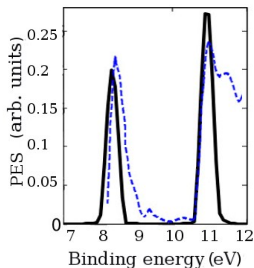
(b) Photoelectron spectrum
