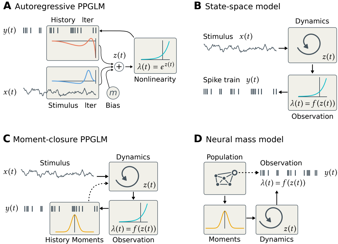
Figure 2: Moment-closure of autoregressive PPGLMs combines aspects of three modeling approaches. A Log-linear autoregressive PPGLM framework (e.g. Weber and Pillow 2017). Dependence on the history of both extrinsic covariates x(t) and the process itself y(t) are mediated by linear filters, which are combined to predict the instantaneous log-intensity of the process. B Latent state-space models learn a hidden dynamical system, which can be driven by both extrinsic covariates and spiking outputs. Such models are often fit using expectation-maximization, and the learned dynamics are descriptive. C Moment-closure recasts autoregressive PPGLMs as state-space models. History dependence of the process is subsumed into the state-space dynamics, but the latent states retain a physical interpretation as moments of the process history (dashed arrow). D Compare to neural mass and neural field models, which define dynamics on a state-space with a physical interpretation as moments of neural population activity.
